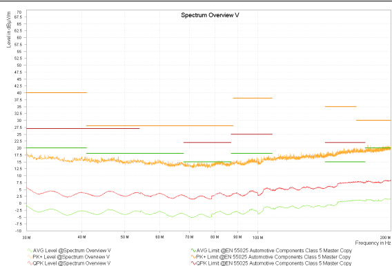
V IN = 12V V OUT = 3.3V F SW = 2MHz I OUT = 4A
