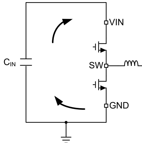
図 8-14. Current Loops With Fast Edges
