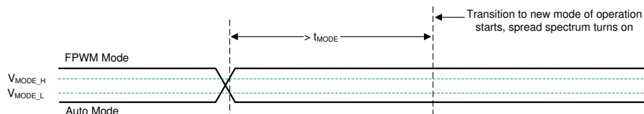
図 7-4. Transition from Auto Mode and FPWM Mode
