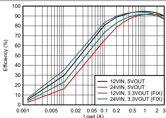
図 8-6. LMR66430MB3RBXNEP Efficiency (Mode = FPWM)
