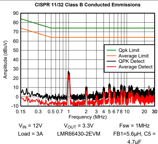
8-13. CISPR 11/32, Class B, Conducted EMI
