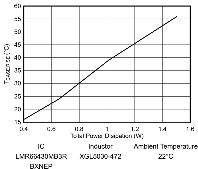
8-12. LMR66430-2EVM Thermal Performance
