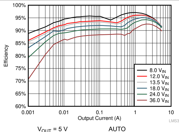
Figure 9-5. Efficiency
