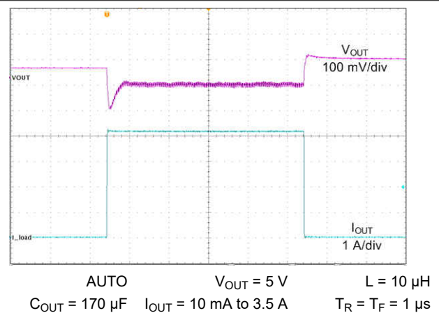
FIG 9-14. Load Transients
