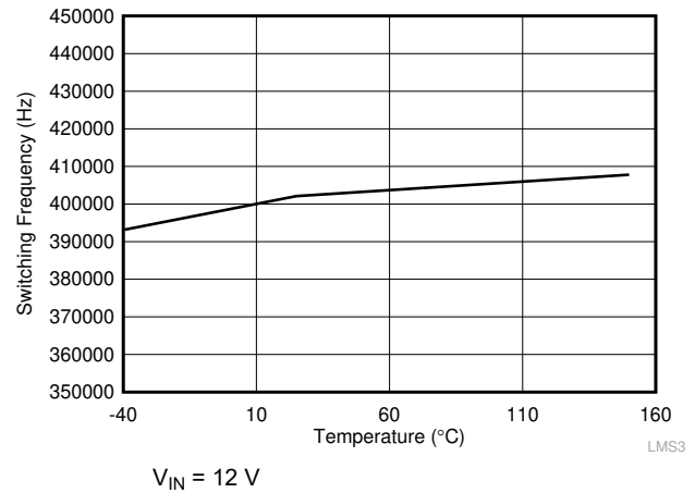
7-2. Switching Frequency vs Temperature
