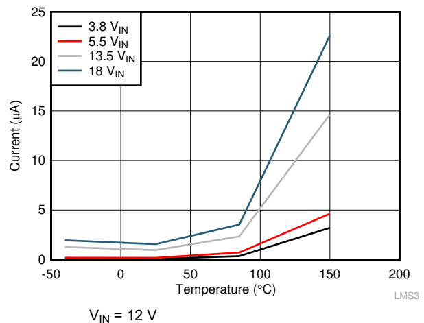
7-6. Shutdown Current
