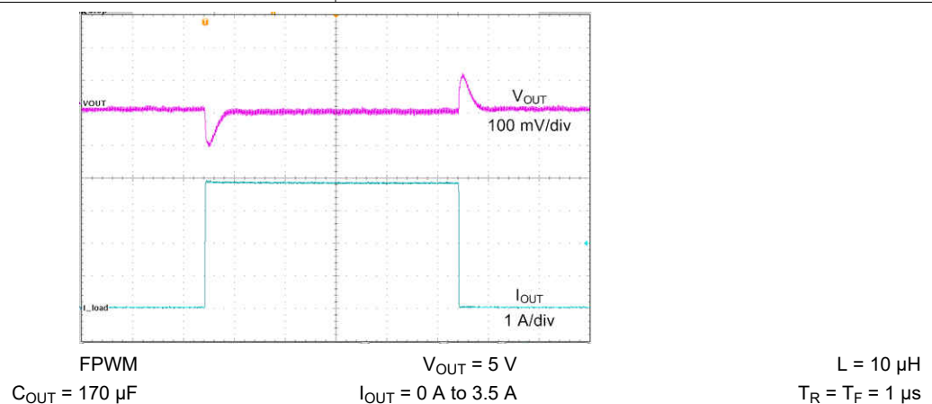
FIG 9-15. Load Transient
