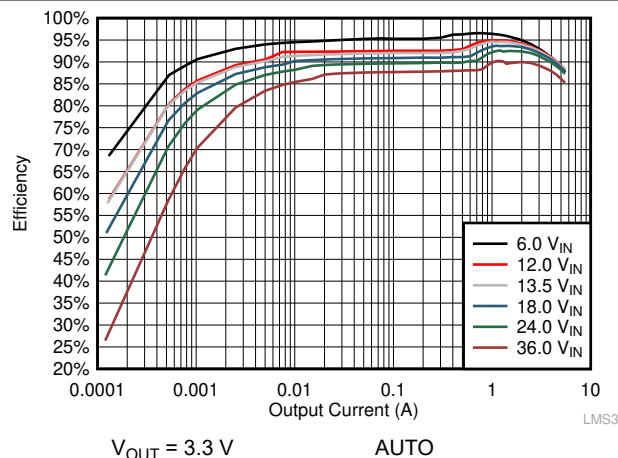
9-17. Efficiency
