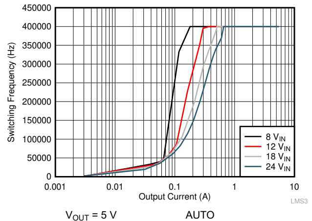
FIG 9-12. Switching Frequency vs Load Current
