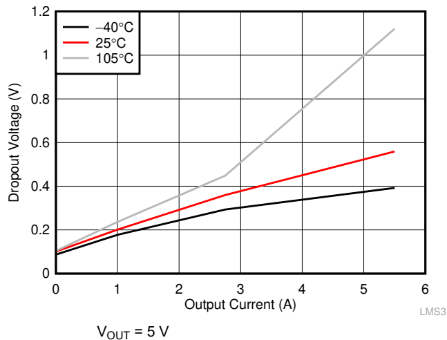
FIG 9-11. Dropout for \geq 330\text{ kHz}
