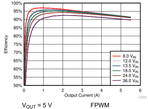
Figure 9-6. Efficiency
