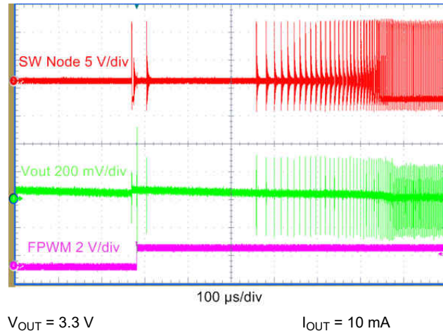
図 9-29. Mode Change Transient AUTO to FPWM mode
