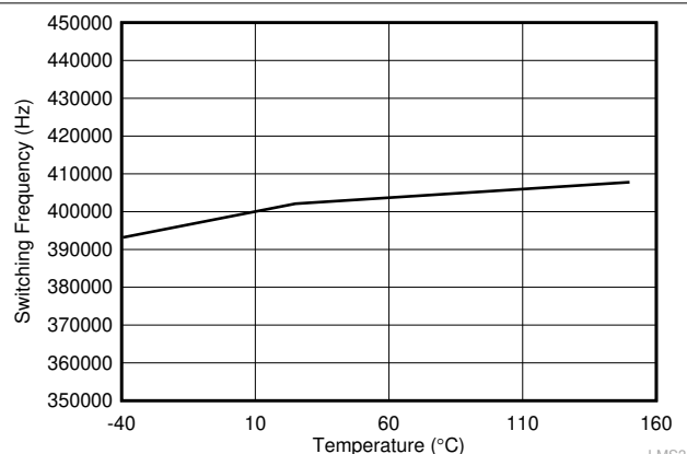
7-2. Switching Frequency vs Temperature
