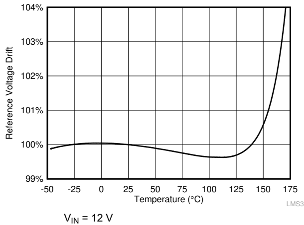
7-1. Reference Voltage Drift
