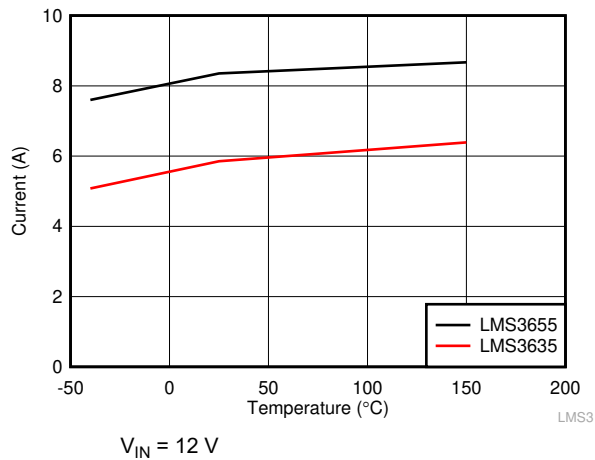
7-3. High-Side/Peak Current Limit for LMS36x5-Q1
