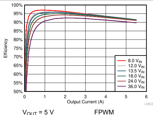
Figure 9-6. Efficiency
