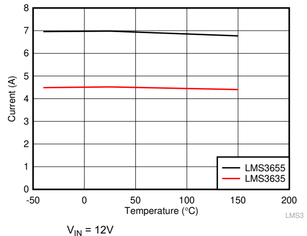
7-4. Low-Side/Valley Current Limit for LMS36x5-Q1
