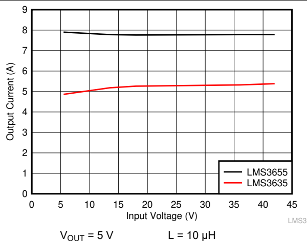
FIG 9-13. Output Current Level Limit Before Overcurrent Protection
