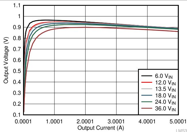
9-18. Efficiency
