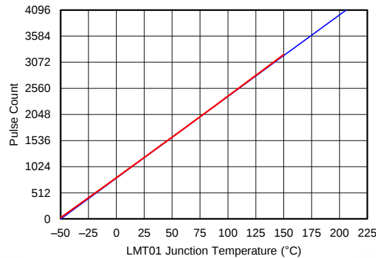
Figure 23. LMT01 Output Transfer Function
