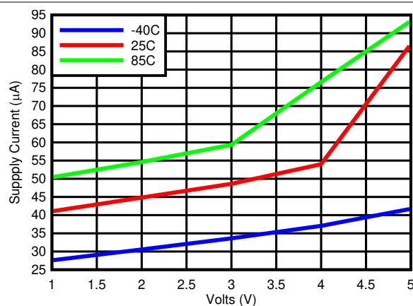
FIG 5-2. Supply Current vs Supply Voltage Output Low
