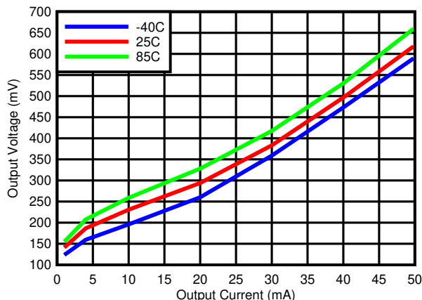
FIG 5-3. Output Voltage vs Output Current
