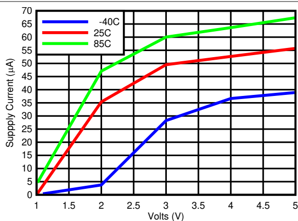
FIG 5-1. Supply Current vs Supply Voltage Output High
