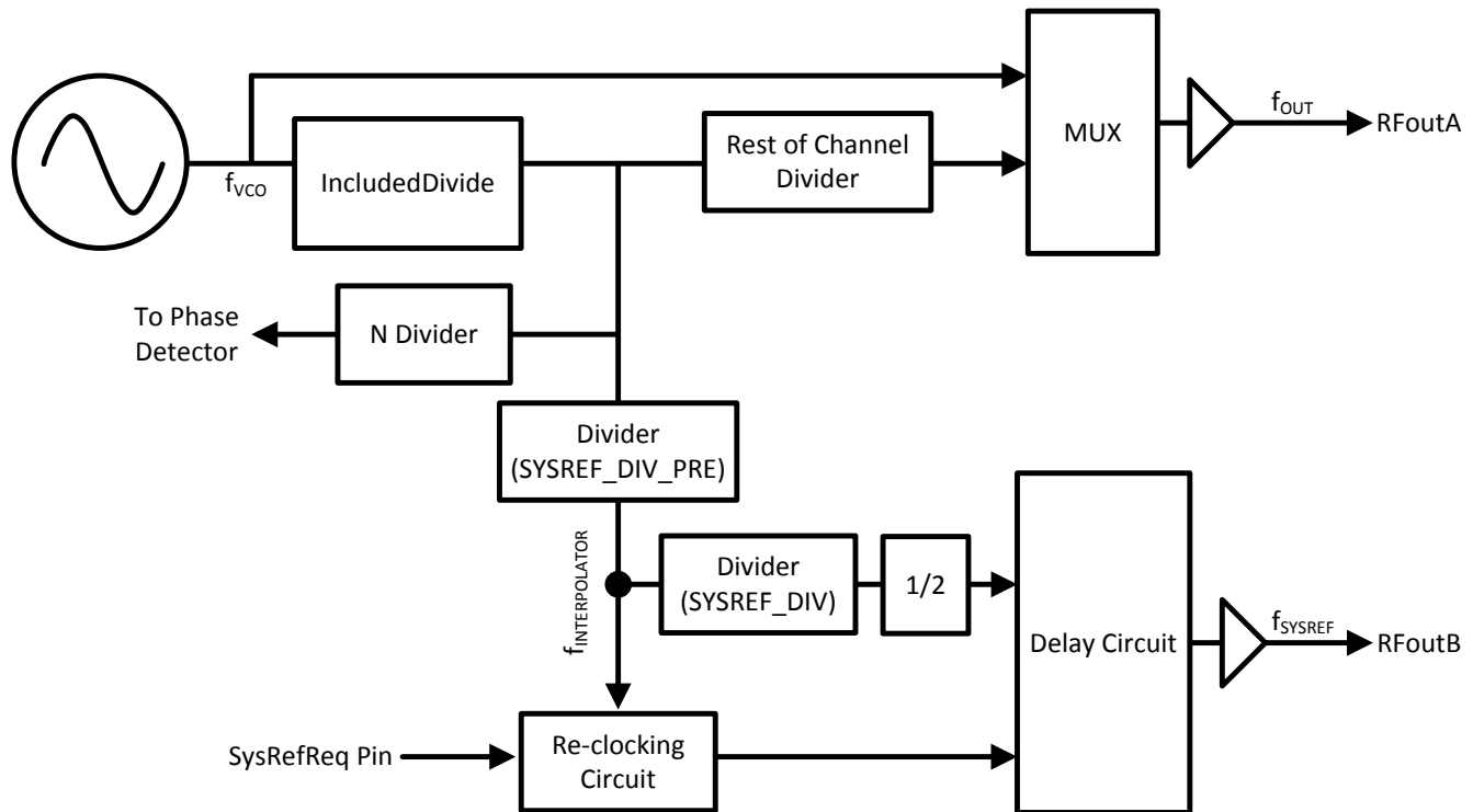
Figure 30. SYSREF Setup
