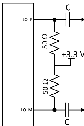
FIG 46. LO Port Operating In Output Mode Requires Load Resistors Or Inductors
