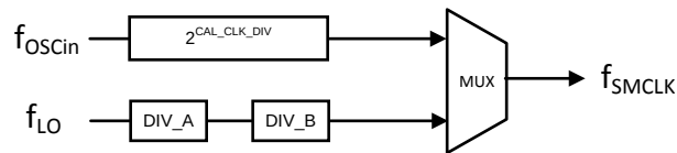
FIG 49. Block Diagram of SM Clock
