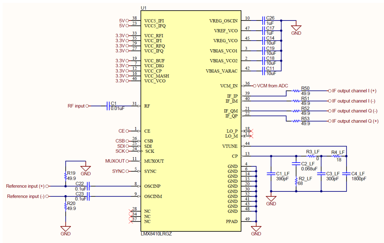
91. Typical Application Schematic
