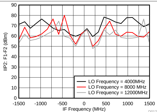
FIG 12. IIP2: F1-F2 Across LO Frequency for External LO Mode
