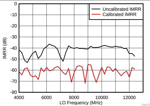
FIG 27. IMRR for Internal LO Mode: Calibrated and Uncalibrated
