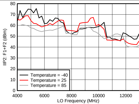
FIG 15. IIP2: F1+F2 Across LO Frequency for Internal LO Mode
