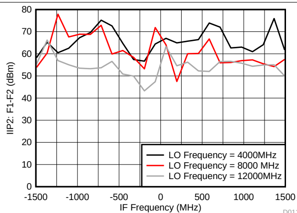
FIG 11. IIP2: F1-F2 Across LO Frequency for Internal LO Mode
