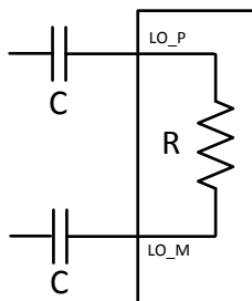
✎ 47. LO Port Operating In Input Mode
