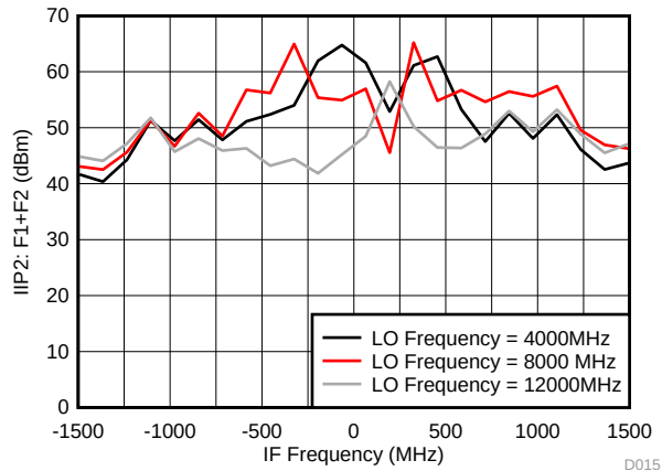
FIG 15. IIP2: F1+F2 Across LO Frequency for Internal LO Mode
