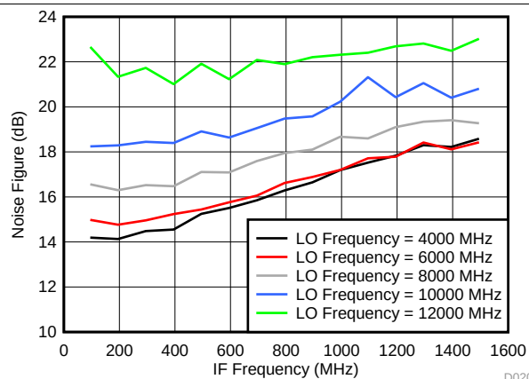
FIG 22. Noise Figure Across IF Frequency for External LO Mode
