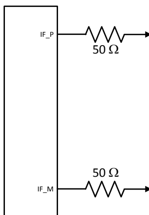
✎ 48. IF Interface Requires External Resistors for 100Ohm Differential Matching
