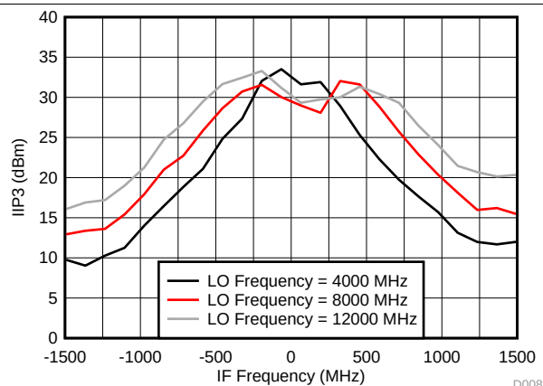
FIG 10. IIP3 Across IF Frequency for External LO Mode
