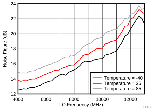
FIG 19. Noise Figure Across LO Frequency for Internal LO Mode
