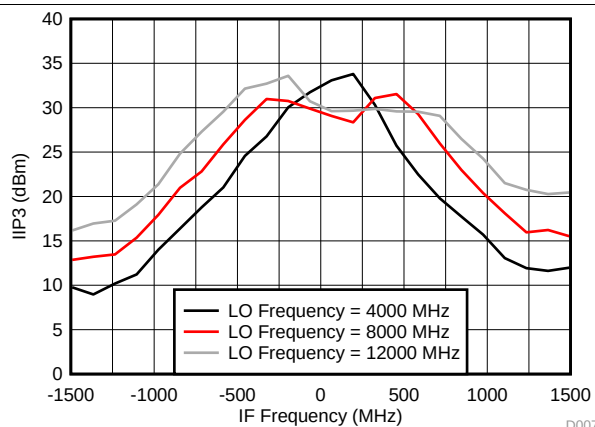
FIG 9. IIP3 Across IF Frequency for Internal LO Mode
