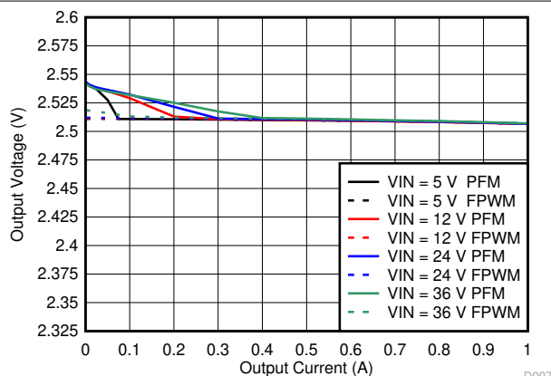
8-34. Line and Load Regulation
