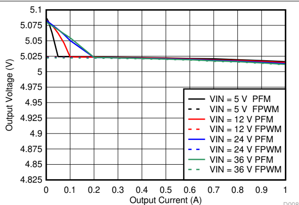
8-10. Line and Load Regulation
