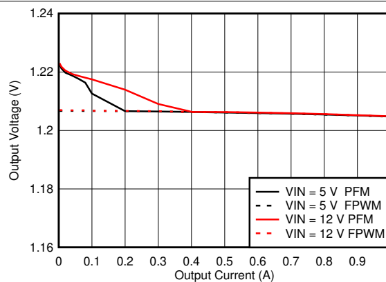
Figure 8-39. Line and Load Regulation for V_{OUT} = 1.2\text{ V}
