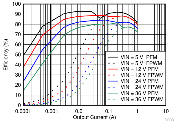
8-12. Efficiency
