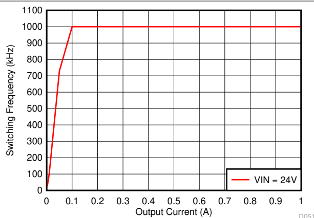
6-29. Auto PFM Mode Switching Frequency vs Output Current
