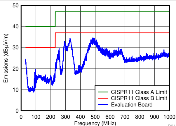
Figure 6-8. Radiated EMI
