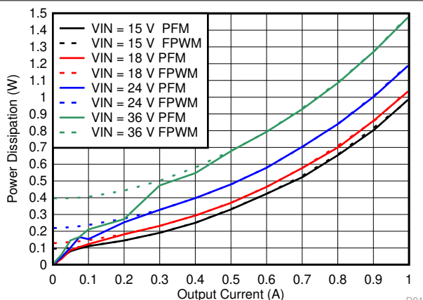
Figure 6-11. Power Dissipation
