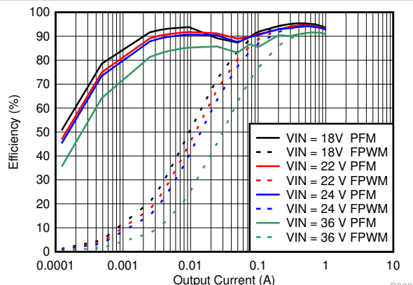
Figure 8-24. Efficiency
