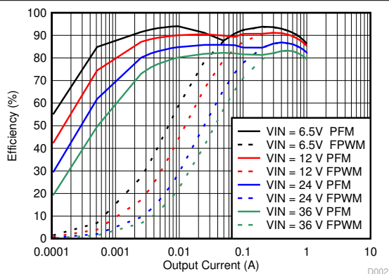
8-6. Efficiency
