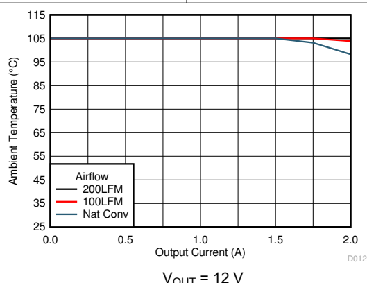
6-13. Safe Operating Area
