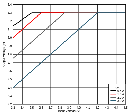
Figure 20. Voltage Dropout
