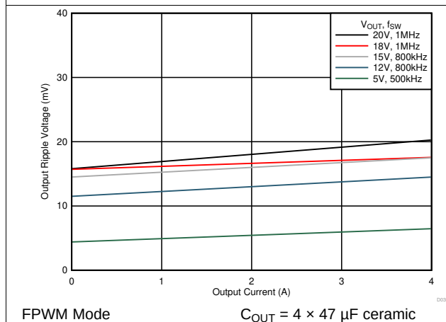
Figure 25. Output Voltage Ripple
