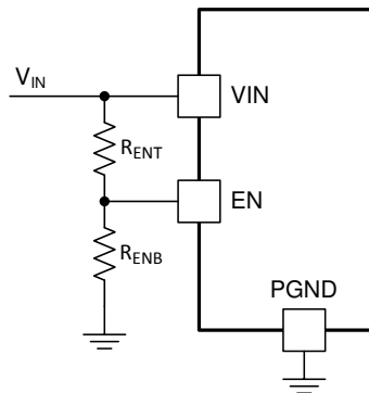
35. System UVLO
