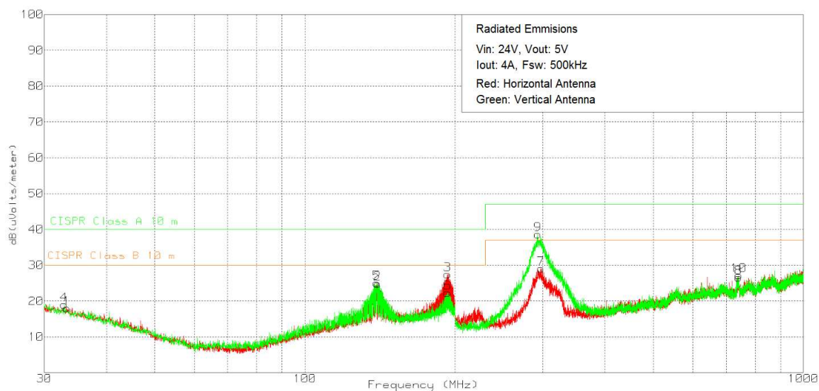
✎ 55. Radiated Emissions 24-V Input, 5-V Output, 4-A Load
