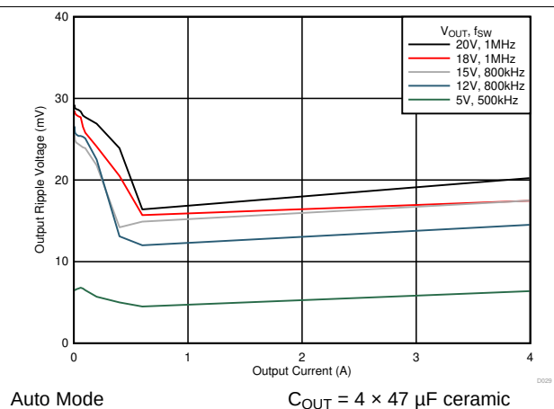
Figure 26. Output Voltage Ripple
