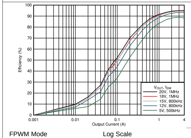
Figure 23. Efficiency vs Output Current
