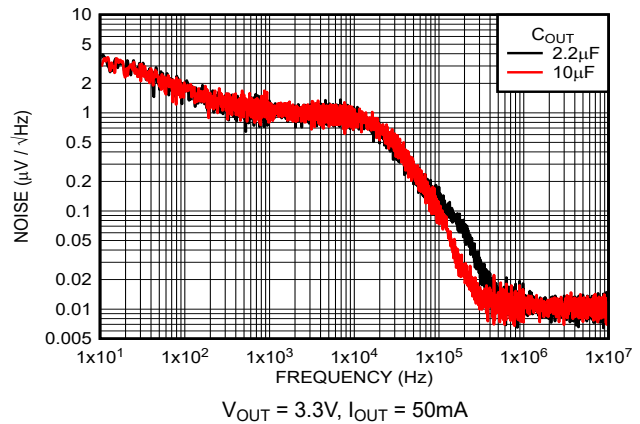
图 5-26. Output Noise Density vs C_{OUT} (New Chip)
