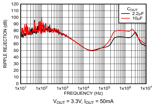
图 5-29. Ripple Rejection vs C_{OUT} (New Chip)
