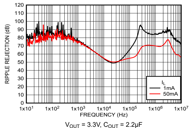
图 5-30. Ripple Rejection vs I_{OUT} (New Chip)
