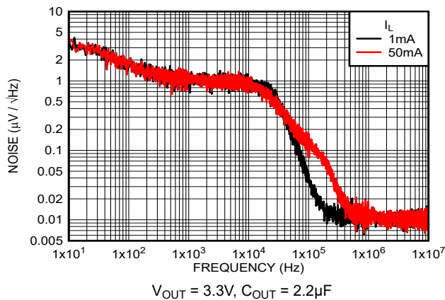
图 5-27. Output Noise Density vs I_{OUT} (New Chip)
