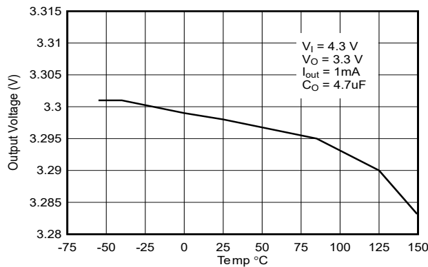
5-1. Output Voltage vs Temperature for Legacy Chip
