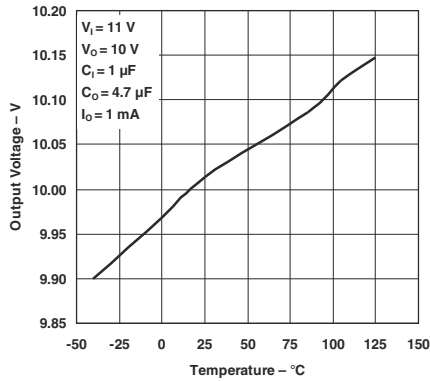
5-1. Output Voltage vs Temperature for Legacy Chip
