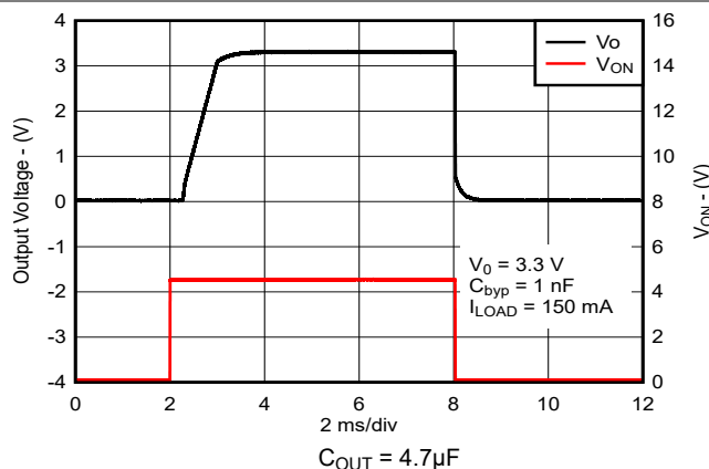
5-56. Turn-On Time (New Chip)
