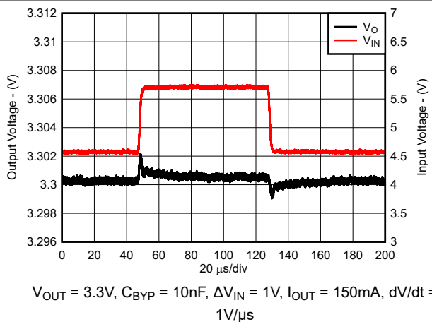
5-50. Line Transient Response (New Chip)
