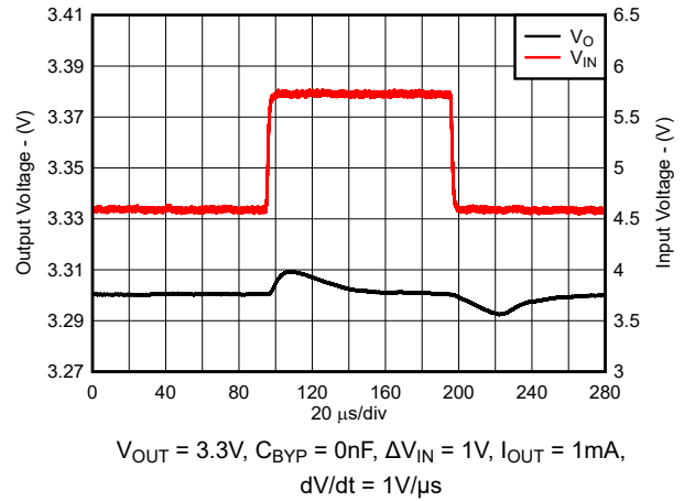
5-44. Line Transient Response (New Chip)
