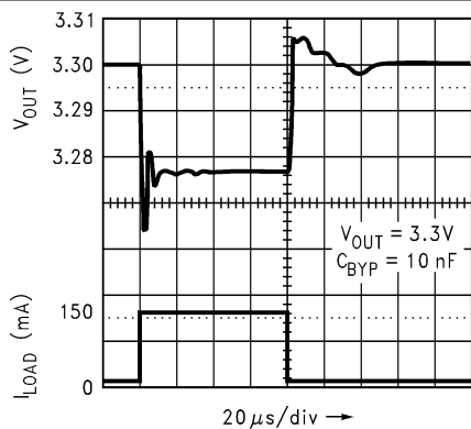
図 7-3. Load Transient Response for Legacy Chip
