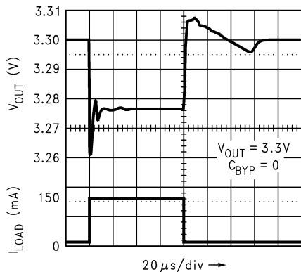
図 7-3. Load Transient Response for Legacy Chip
