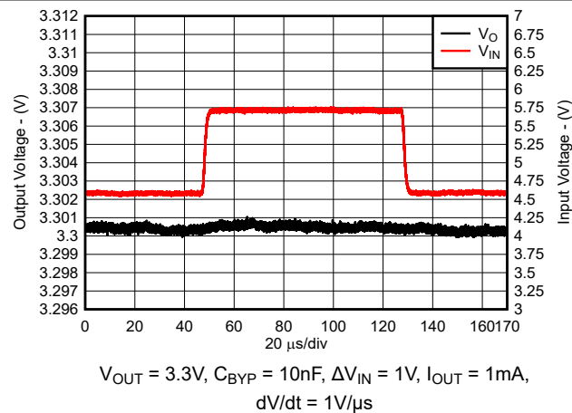
5-48. Line Transient Response (New Chip)
