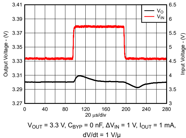
図 7-8. Line Transient Response for New Chip
