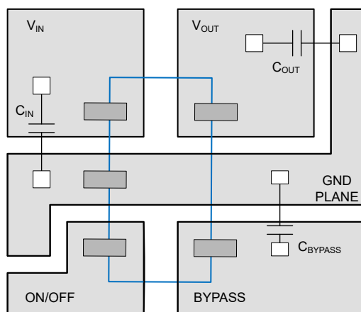
✎ 7-15. Layout Diagram
