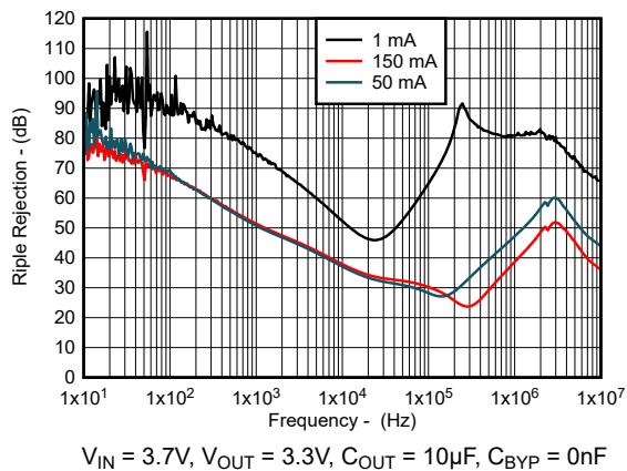
Figure 5-17. Ripple Rejection vs Frequency (New Chip)
