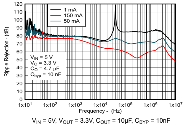
Figure 5-20. Ripple Rejection vs Frequency (New Chip)
