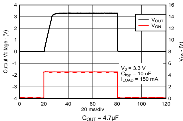
5-58. Turn-On Time (New Chip)
