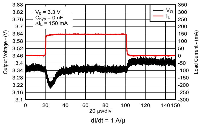
図 7-6. Load Transient Response for New Chip
