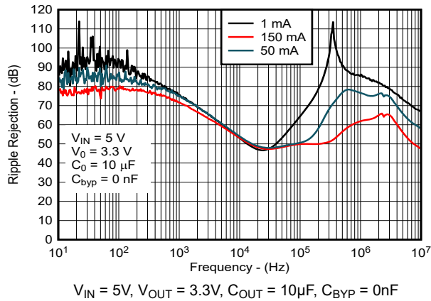
Figure 5-13. Ripple Rejection vs Frequency (New Chip)
