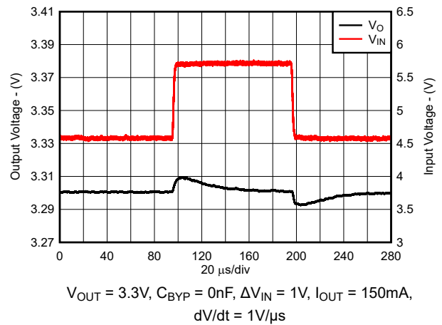
5-46. Line Transient Response (New Chip)
