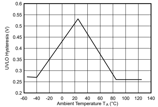
Figure 6-4. V_{CC} UVLO Hysteresis
