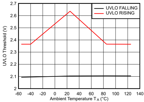
Figure 6-3. V_{CC} UVLO Rising and Falling Thresholds
