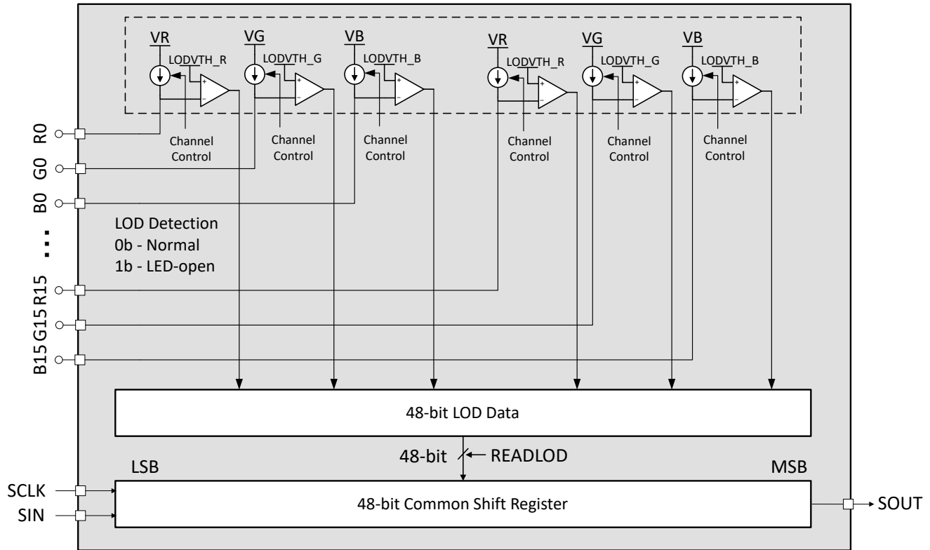
7-8. LED Open Detection Circuit
