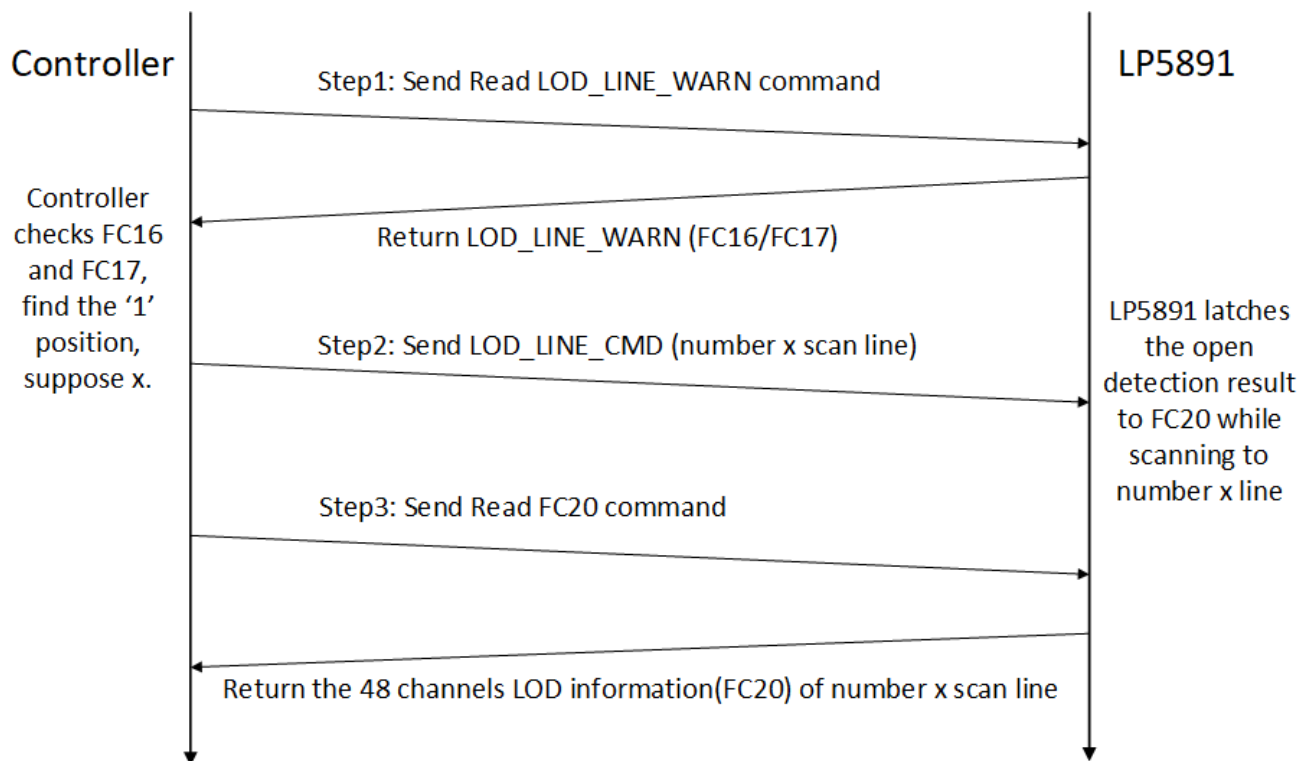
FIG 7-10. Steps to Read LED Open Information
