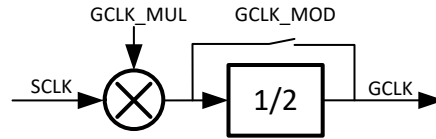
7-6. Frequency Multiplier Block Diagram
