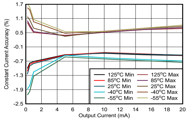
FIG 6-5. Channel to Channel Accuracy vs Output Current
