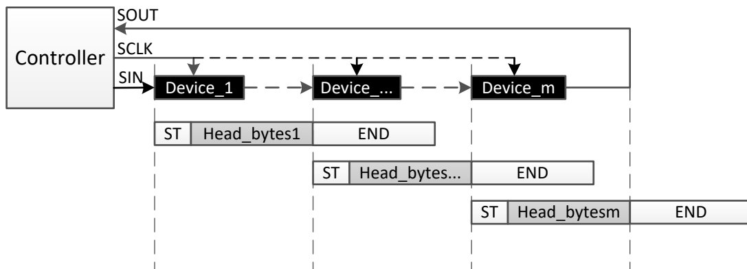
☒ 7-18. Chip Index Write Command
