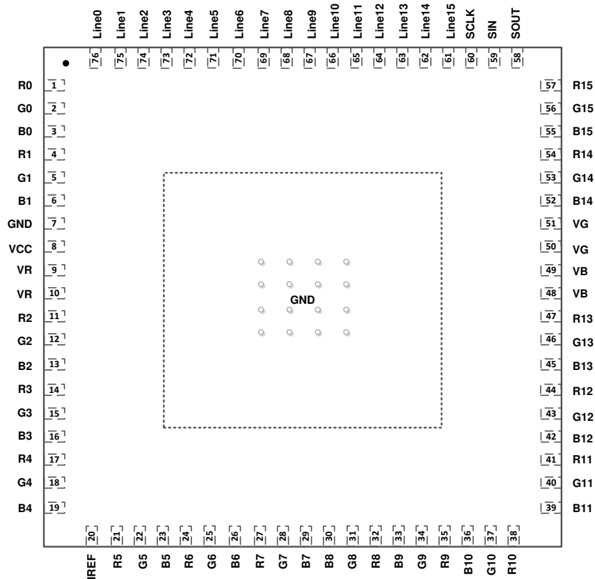
5-1. LP5891 RRF Package 76-Pin VQFN With Exposed Thermal Pad Top View
