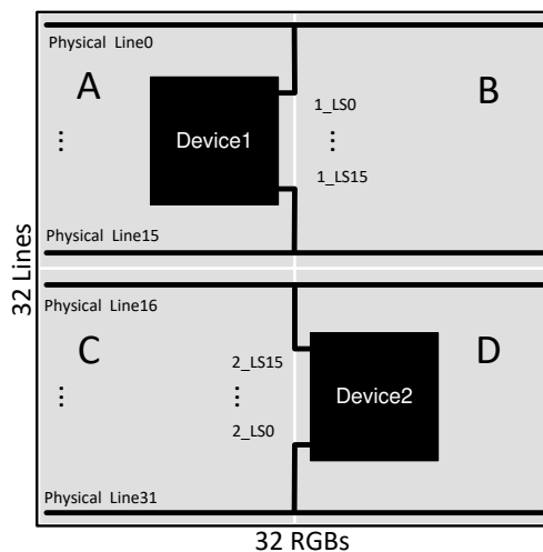
7-2. Mode2 Diagram
