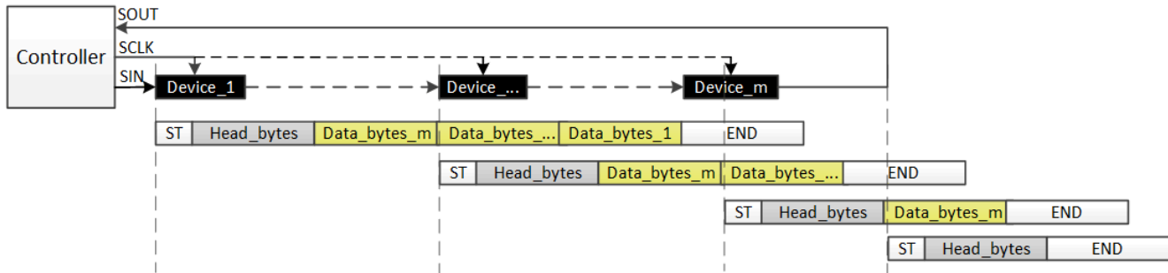
7-23. Data Write Command with Non-Broadcast
