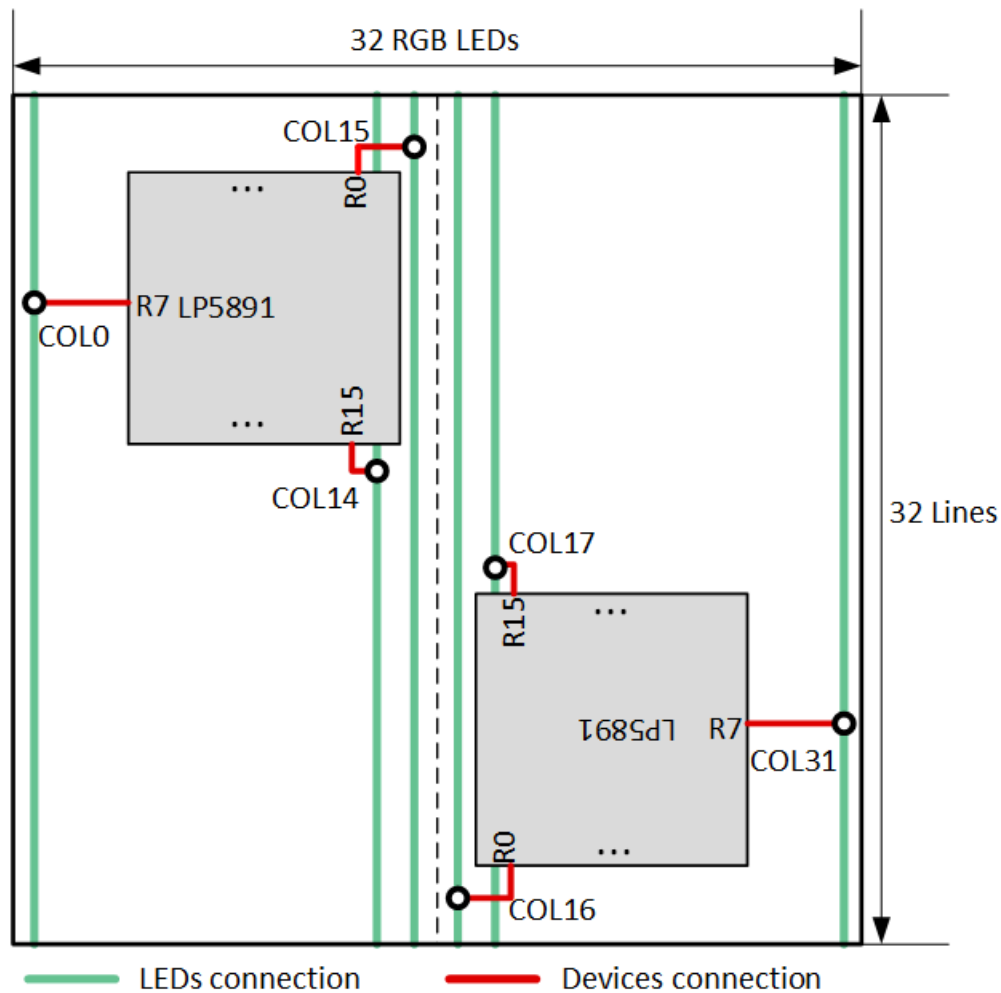
FIG 10-3. Channel Routing Suggestion with Shortest Wire
