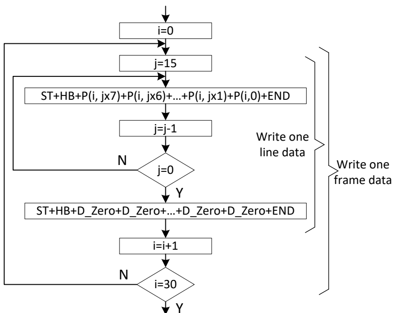
8-4. Data Write Flow
