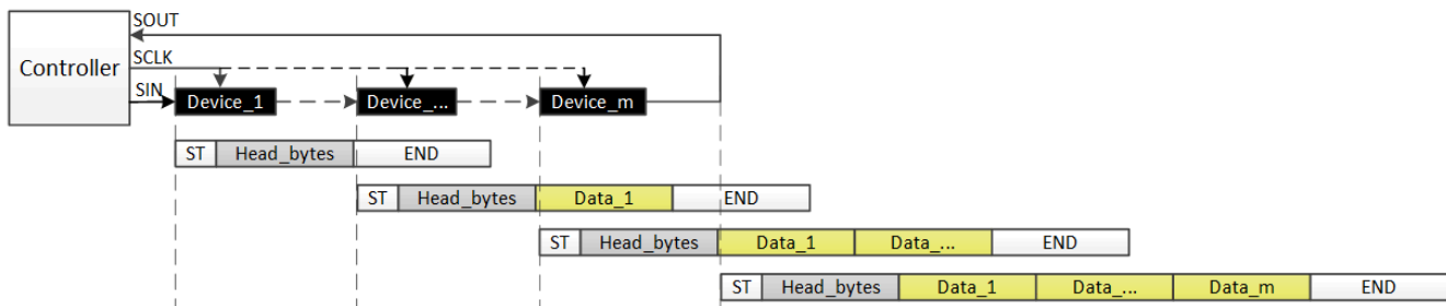
7-25. Data Read Command
