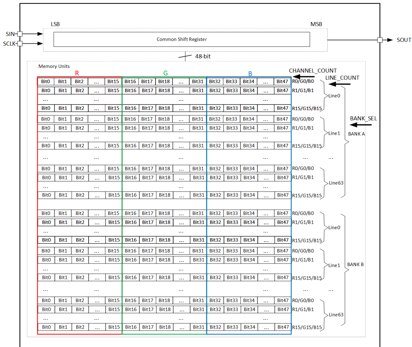
7-27. LP5891 Memory-unit Structure
