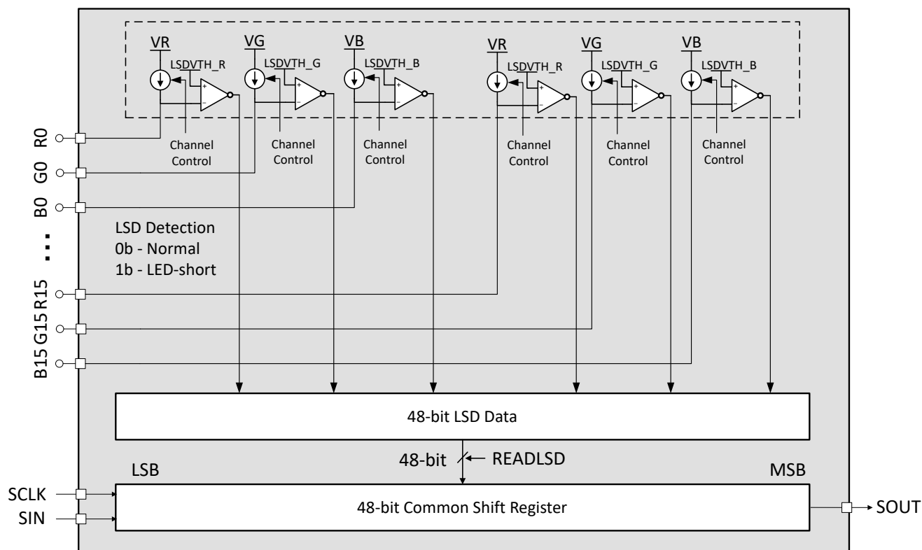
✎ 7-12. LED Short Detection Circuit
