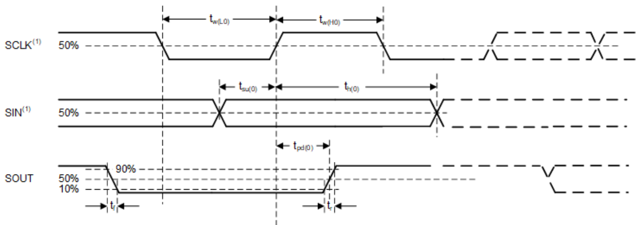
FIG 6-1. Timing and Switching Diagram
