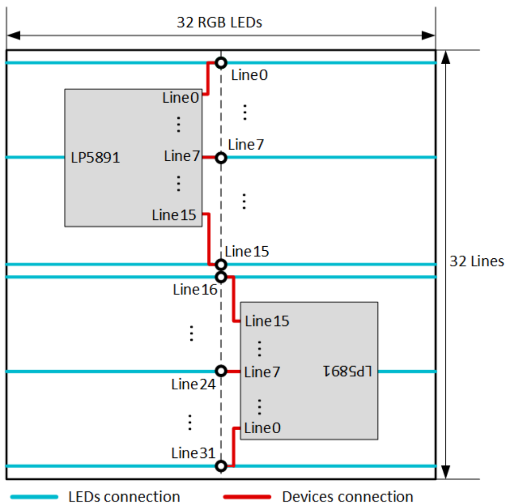
✎ 10-2. Line Routing Suggestion
