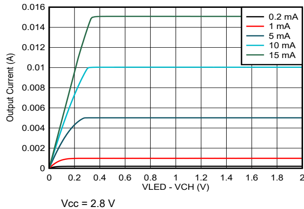
FIG 6-2. Channel Current vs (VLED-Vchannel) Voltage
