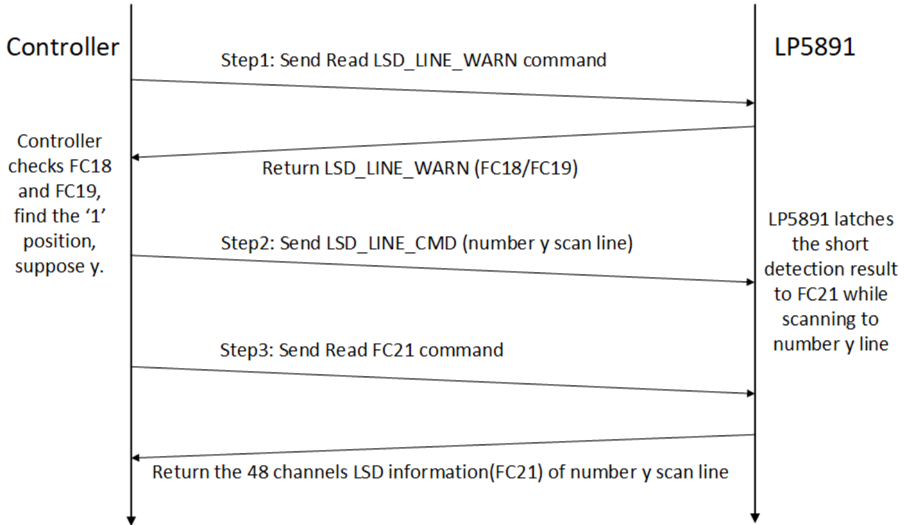
☒ 7-14. Steps to Read LED Short Information
