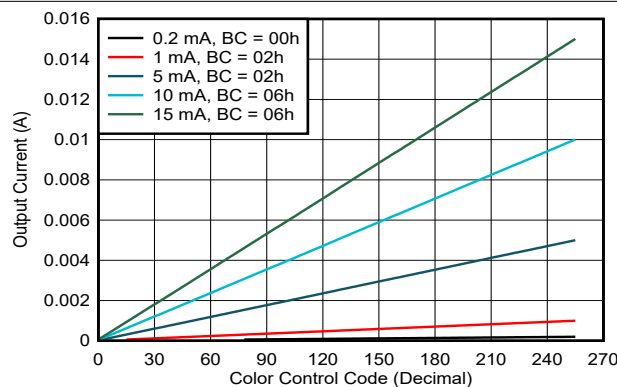
FIG 6-6. Color Control Code vs Output Current
