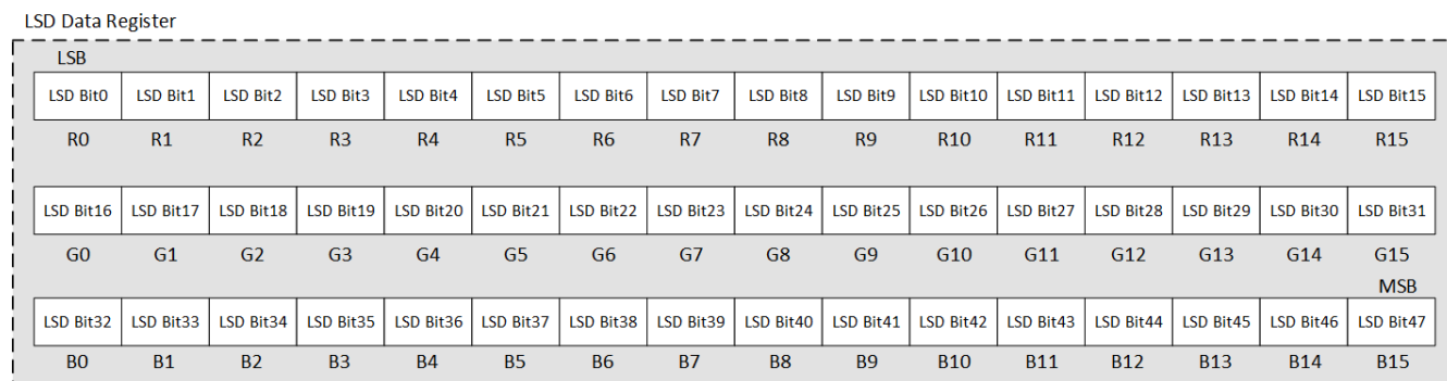
✎ 7-13. Bit Arrangement in the LSD Data Register
