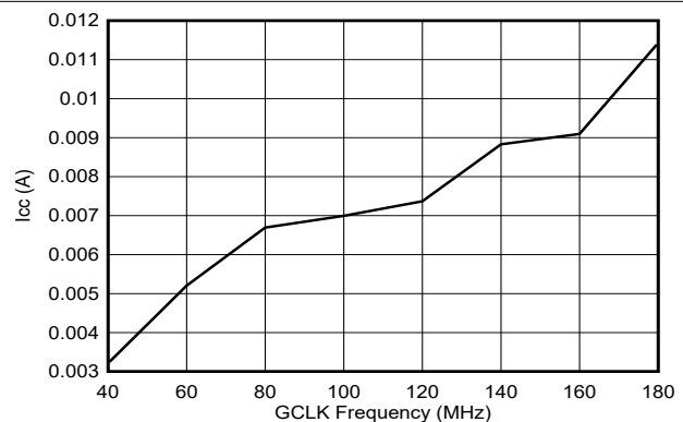
FIG 6-7. I CC Current vs GCLK Frequency
