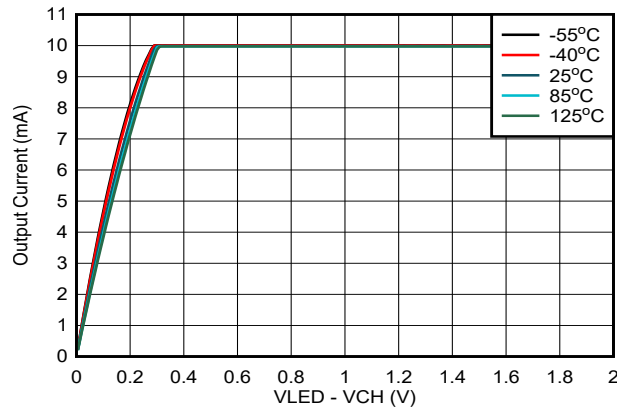
FIG 6-4. Channel Current vs. (VLED-Vchannel) Voltage
