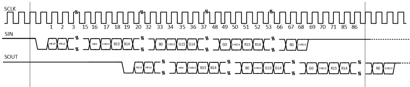
7-22. Data Write Command with Broadcast (Timing Diagram)
