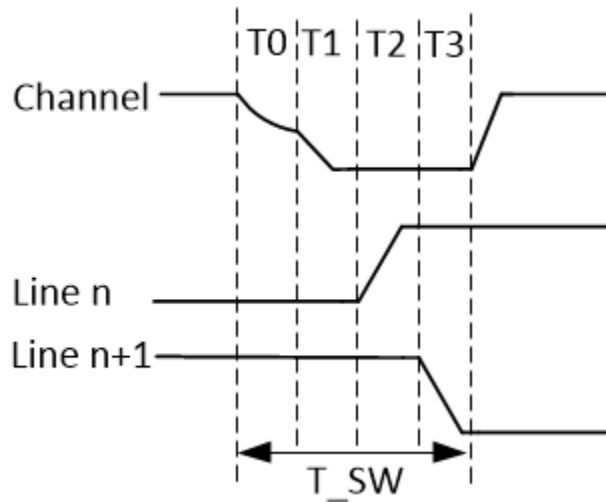
7-7. Line Transitioning Sequence
