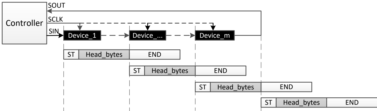
7-19. VSYNC Write Command
