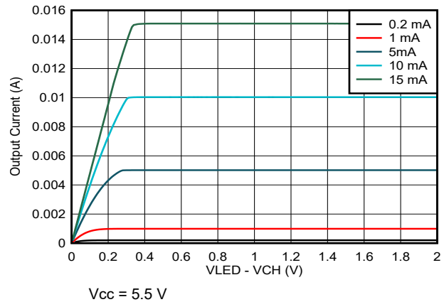
FIG 6-3. Channel Current vs (VLED-Vchannel) Voltage
