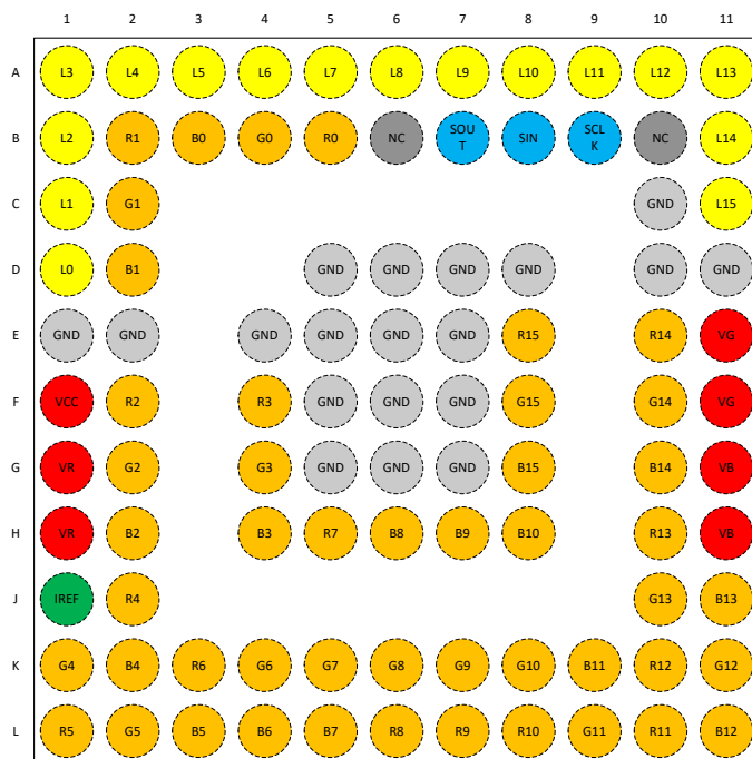
5-2. LP5891 ZXL Package 96-Pin BGA Top View
