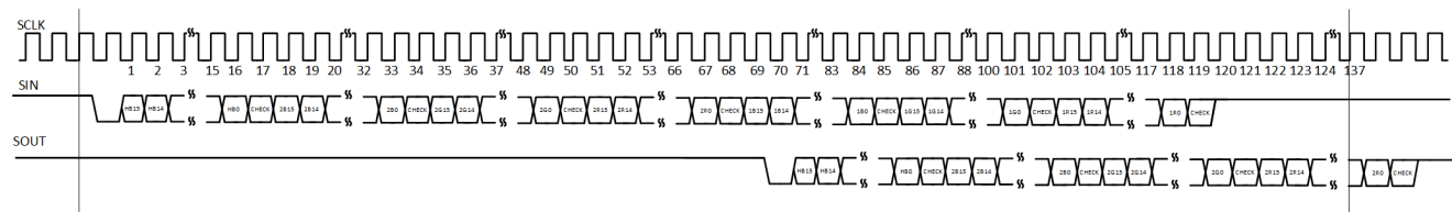
7-24. Data Write Command with Non-Broadcast (Timing Diagram)
