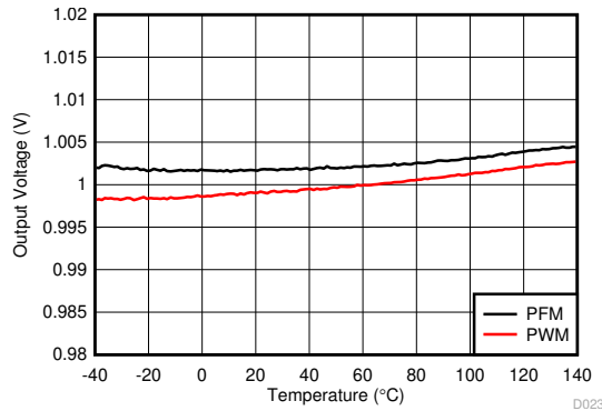
✎ 8-16. Buck Output Voltage vs Temperature
