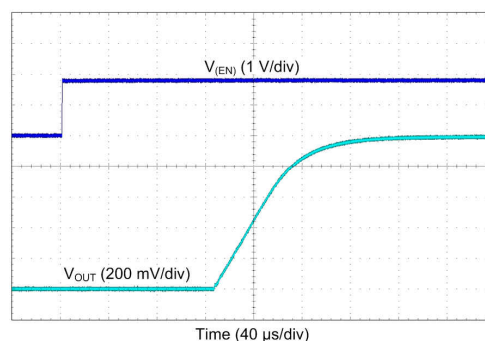
图 8-45. LDO Start-Up
