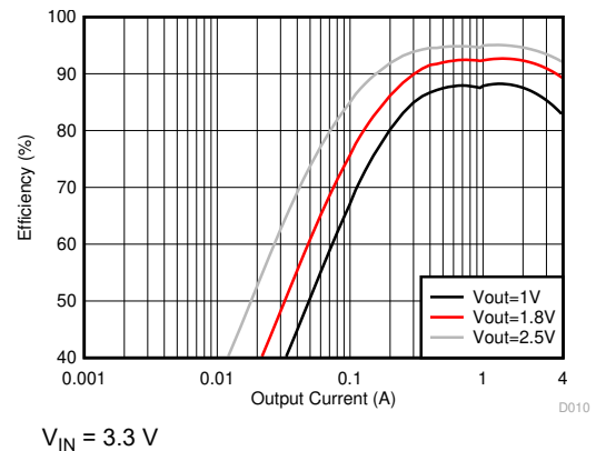
図 8-7. Buck Efficiency in Forced PWM Mode (Dual-Phase Output)
