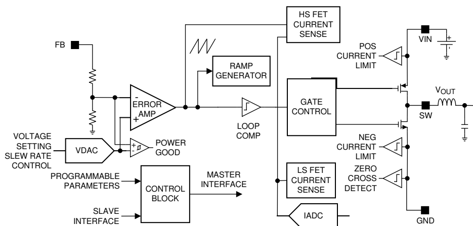
7-1. Detailed Block Diagram Showing One Core
