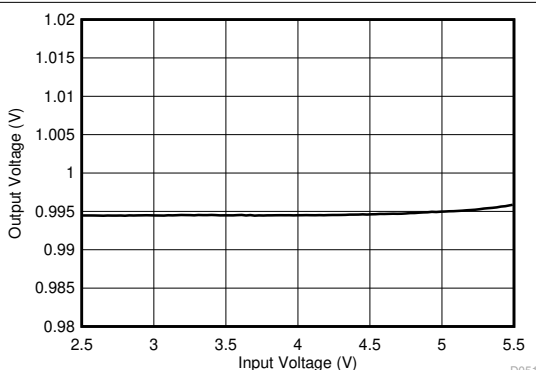
8-22. LDO Output Voltage vs Input Voltage
