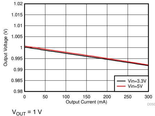
✎ 8-42. LDO Output Voltage vs Load Current
