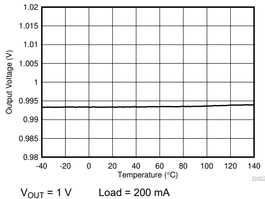
✎ 8-44. LDO Output Voltage vs Temperature
