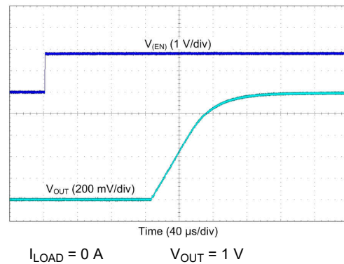
✎ 8-45. LDO Start-Up
