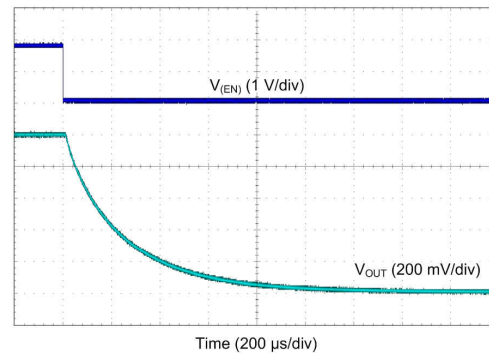
图 8-47. LDO Shutdown
