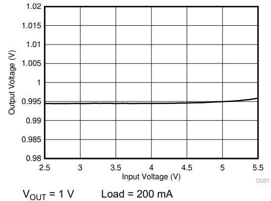
✎ 8-43. LDO Output Voltage vs Input Voltage
