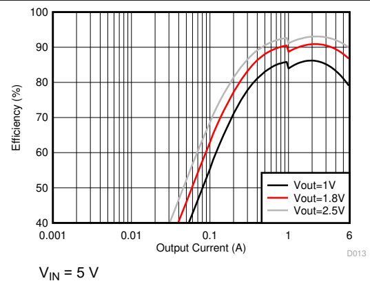
図 8-9. Buck Efficiency in Forced PWM Mode (Dual-Phase Output)
