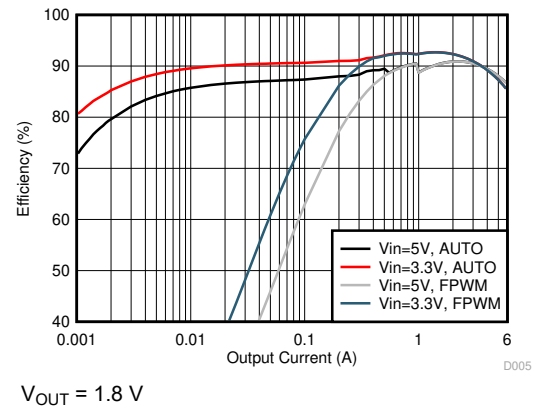
図 8-5. Buck Efficiency in PFM/PWM and Forced PWM Mode (Dual-Phase Output)
