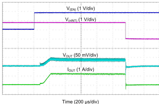
图 8-40. Buck Start-Up With Short on Output (Single-Phase Output)
