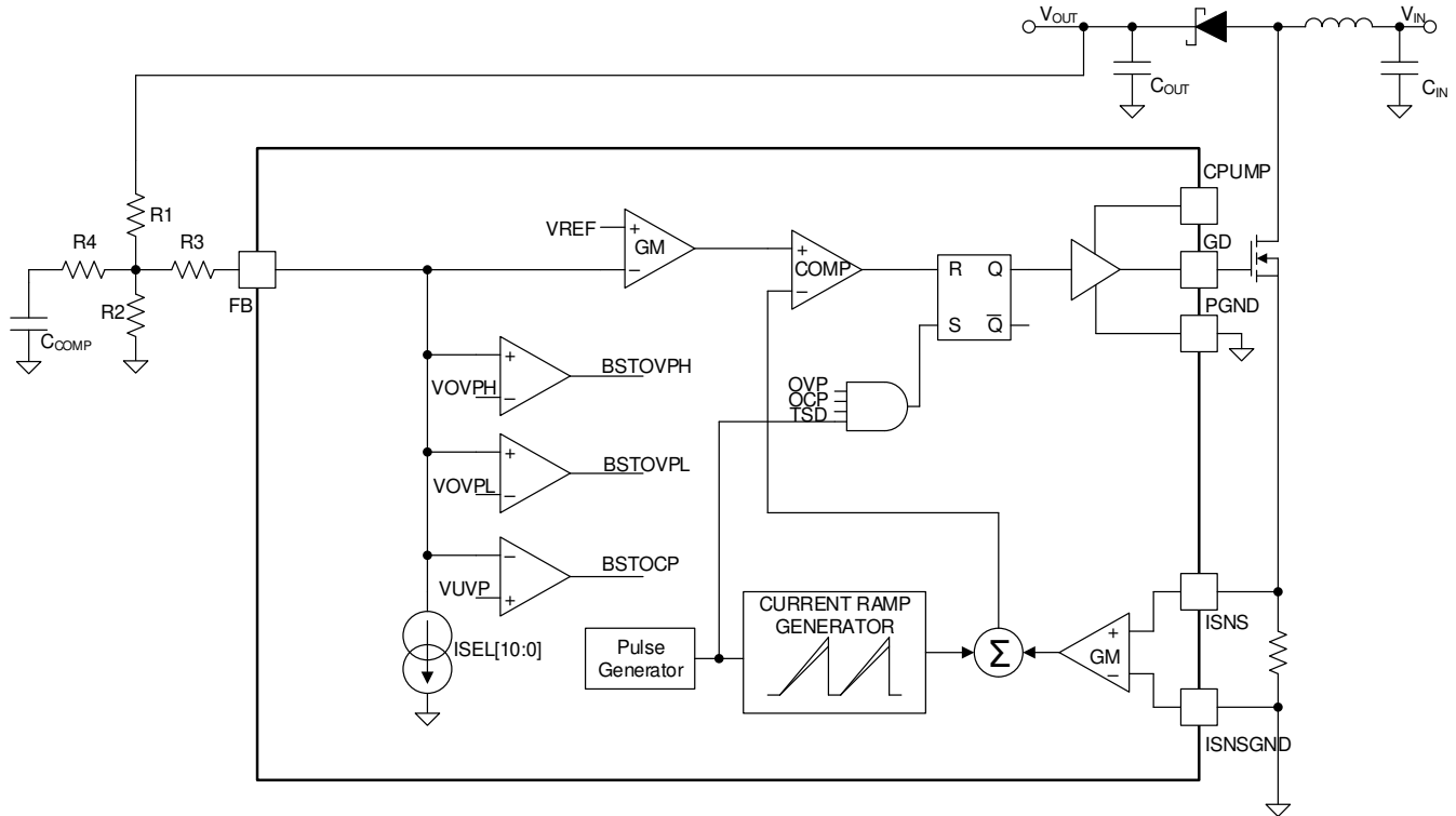
FIG 6-7. External Compensation Network
