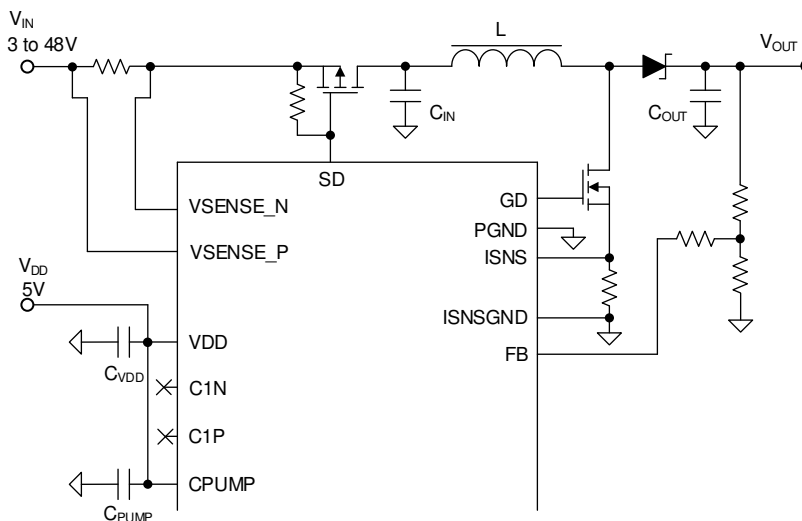
6-2. Charge Pump Disabled Circuit
