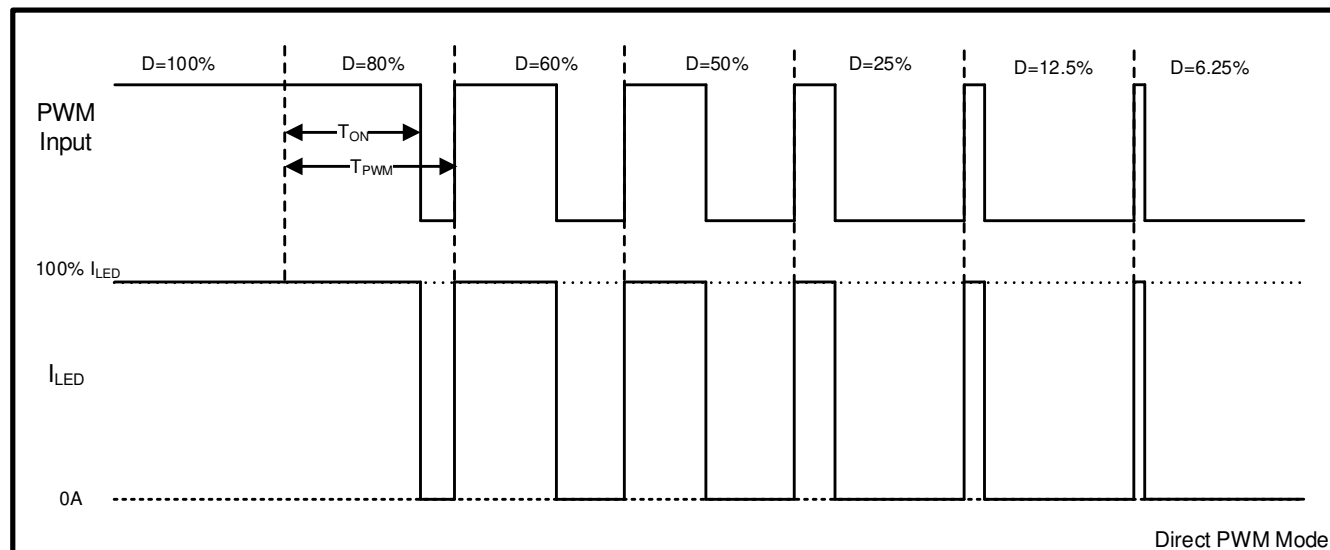
図 6-12. Direct PWM Dimming Diagram
