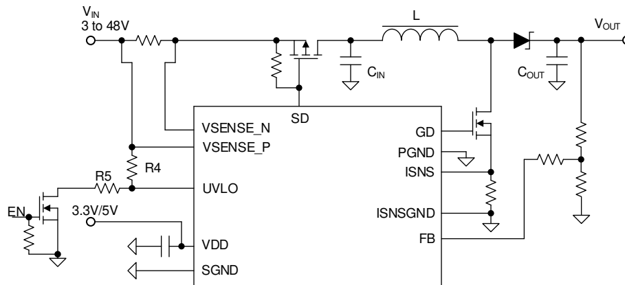
図 6-17. V_{IN} UVLO Setting Circuit Without Current Leakage Path
