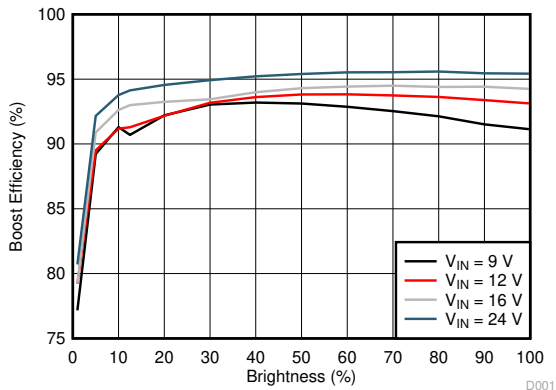
図 5-2. Boost Efficiency
