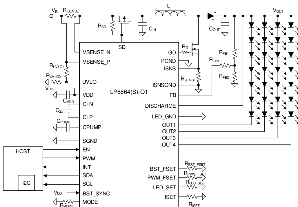
図 7-1. Full Feature Application for Display Backlight
