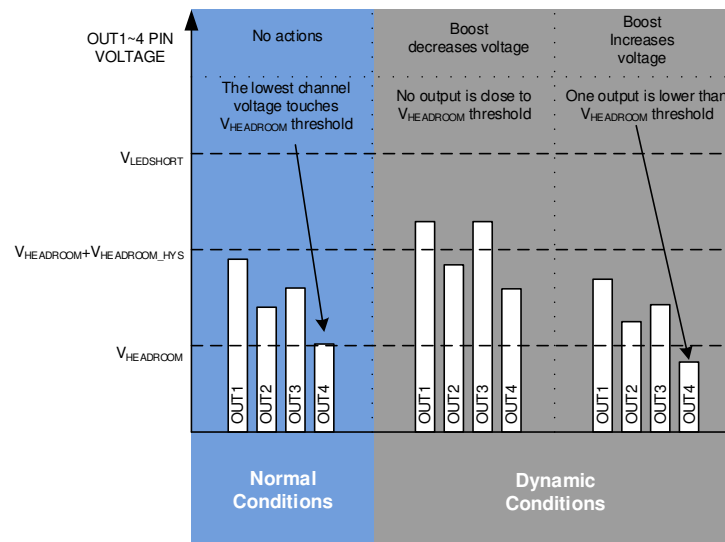
図 6-4. Adaptive Boost Voltage Control Loop Function
