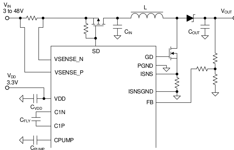
6-1. Charge Pump Enabled Circuit
