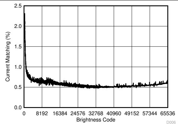
Figure 5-7. Current Matching
