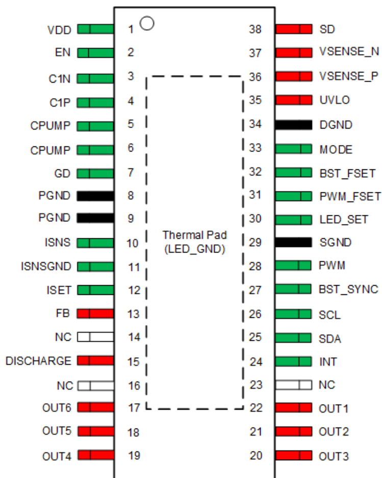
図 4-1. DCP Package 38-Pin HTSSOP Top View
