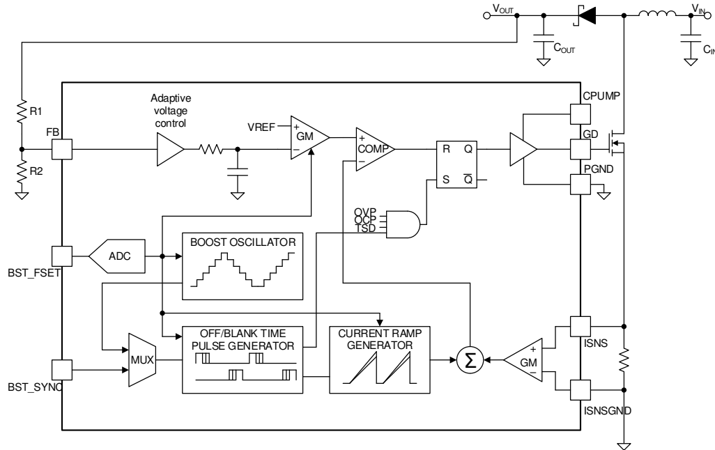
図 6-3. Boost Controller Block Diagram
