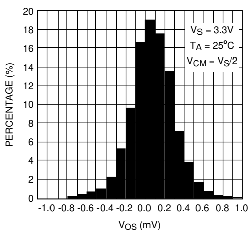
Figure 5-5. Offset Voltage Distribution
