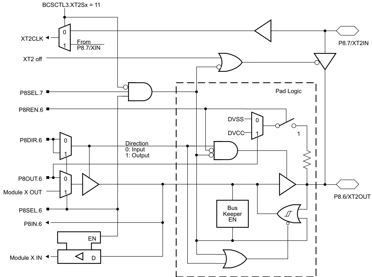
Figure 9-17. Port P8 (P8.6) Diagram
