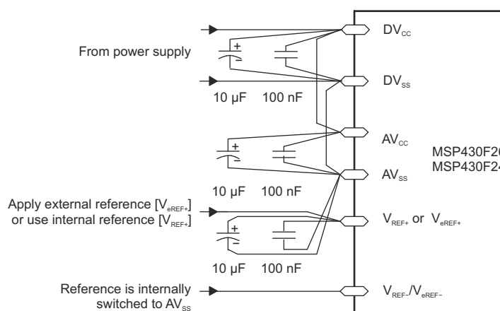
8-40. Supply Voltage and Reference Voltage Design V_{REF}/V_{REF-} = AV_{SS} , Internally Connected
