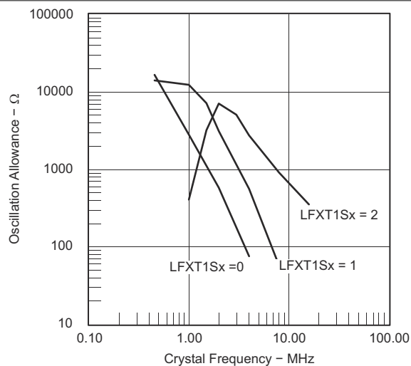
FIG 8-23. Oscillation Allowance vs Crystal Frequency C_{L,eff} = 15 \text{ pF} , T_A = 25^\circ\text{C}
