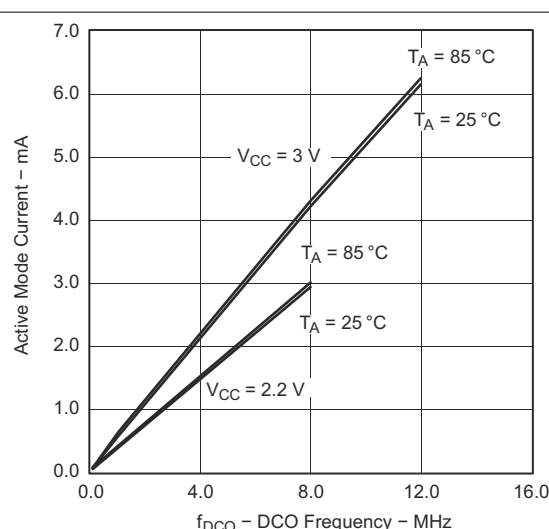
8-3. Active Mode Current vs DCO Frequency
