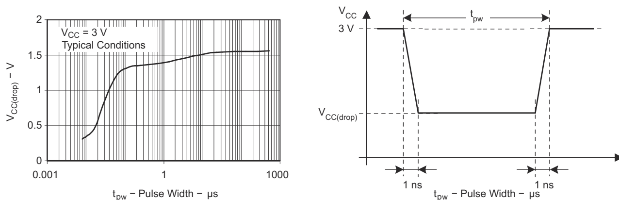
8-10. V_{CC(drop)} Level With a Rectangular Voltage Drop to Generate a POR or BOR Signal
