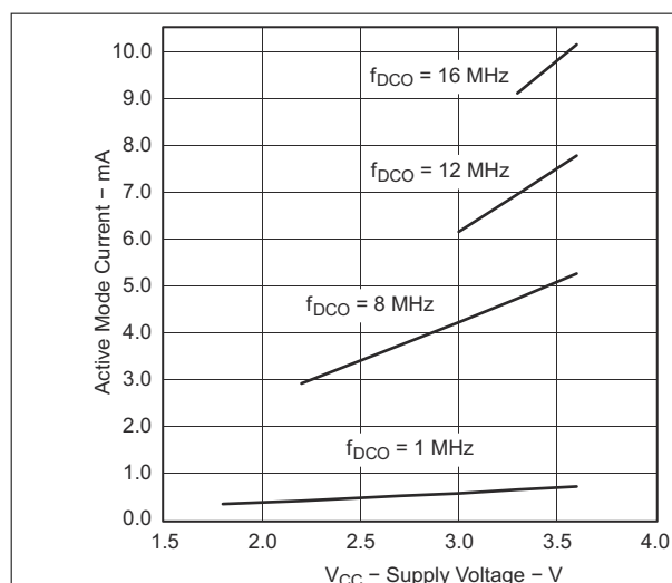
8-2. Active Mode Current vs Supply Voltage ( T_A = 25^\circ\text{C} )
