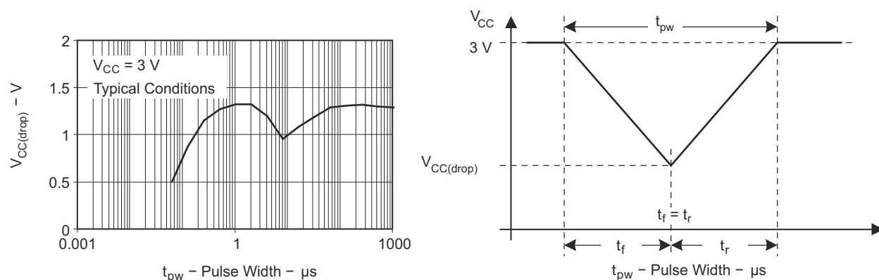
8-11. V_{CC(drop)} Level With a Triangular Voltage Drop to Generate a POR or BOR Signal
