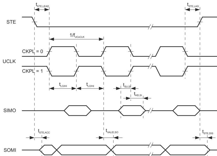
8-29. SPI Slave Mode, CKPH = 0
