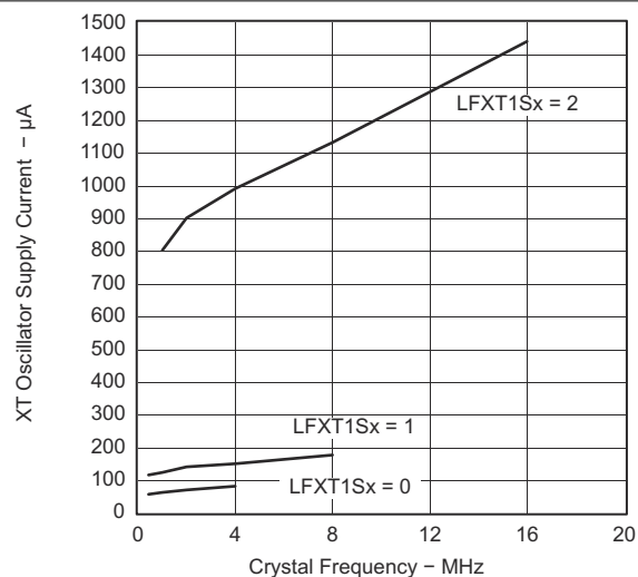
FIG 8-24. Oscillator Supply Current vs Crystal Frequency C_{L,eff} = 15 \text{ pF} , T_A = 25^\circ\text{C}
