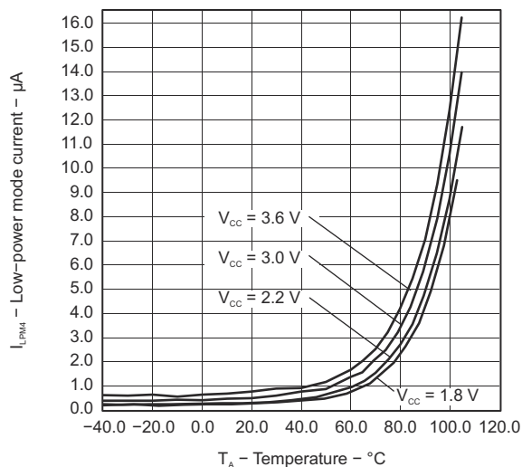
8-4. LPM4 Current vs Temperature
