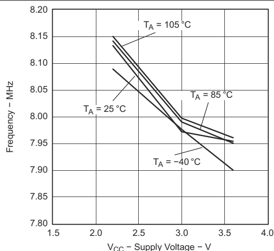
8-15. Calibrated 8-MHz Frequency vs Supply Voltage
