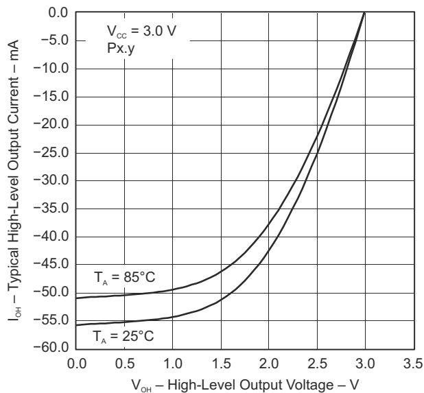
FIG 8-10. Typical High-Level Output Current vs High-Level Output Voltage
