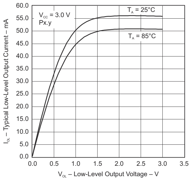
FIG 8-8. Typical Low-Level Output Current vs Low-Level Output Voltage
