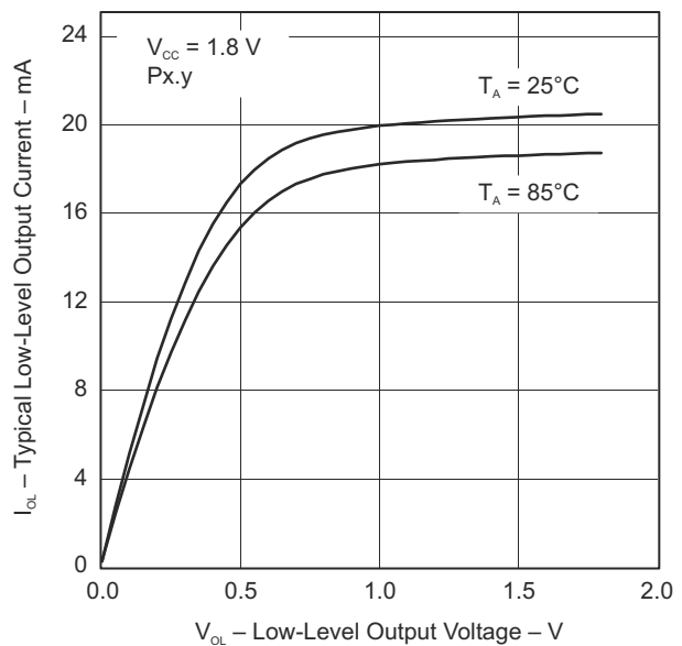
FIG 8-9. Typical Low-Level Output Current vs Low-Level Output Voltage
