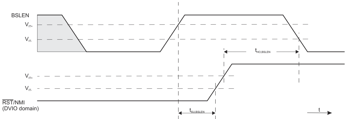
8-18. DVIO BSL Entry Timing
