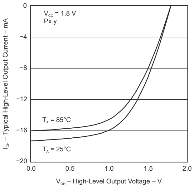
FIG 8-11. Typical High-Level Output Current vs High-Level Output Voltage
