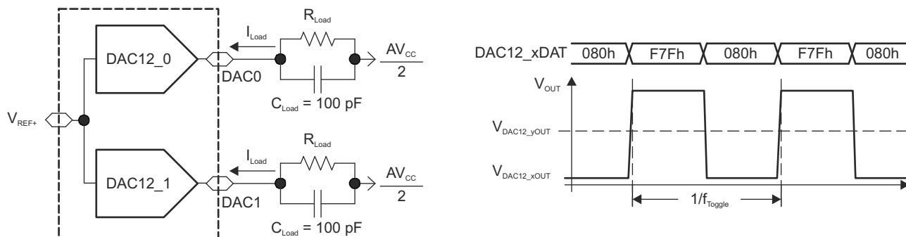
图 8-22. Crosstalk Test Conditions
