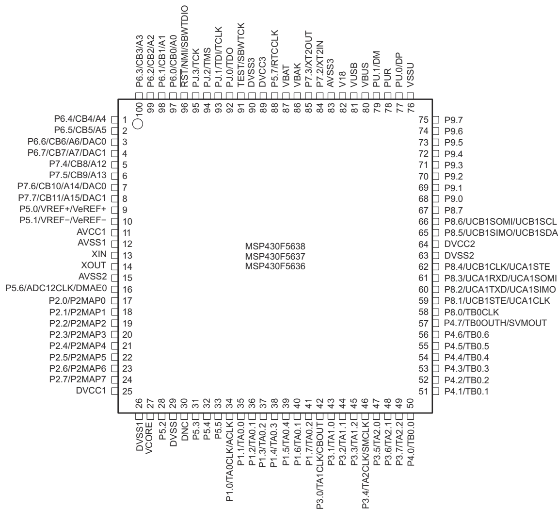
7-1. 100-Pin PZ Package (Top View) – MSP430F5638, MSP430F5637, MSP430F5636
