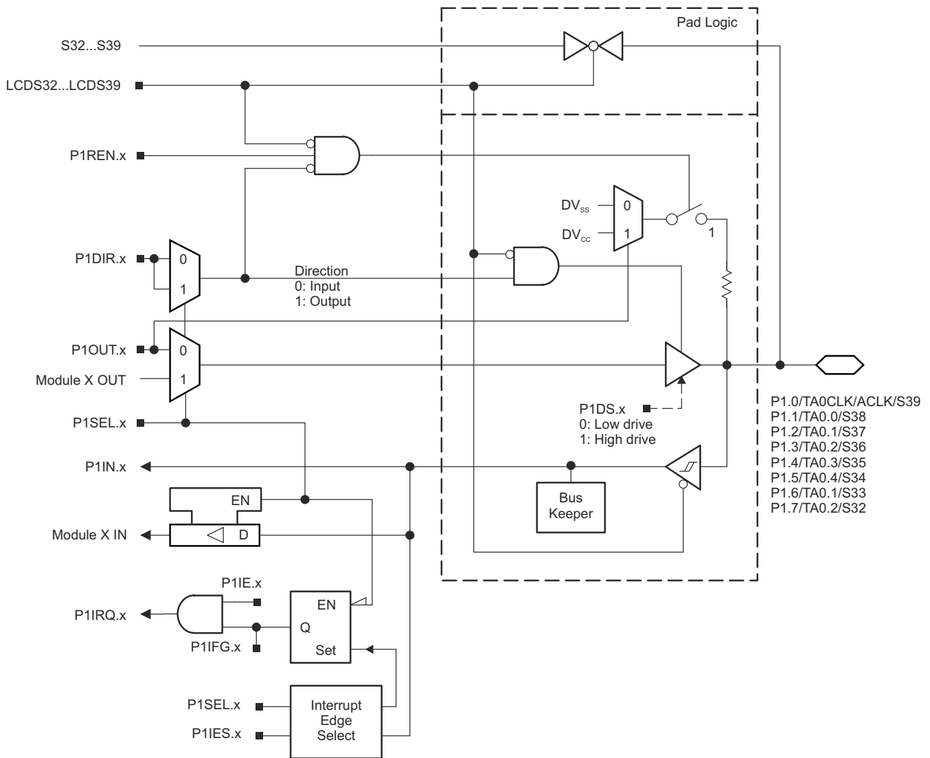
❏ 9-2. Port P1 (P1.0 to P1.7) Diagram
