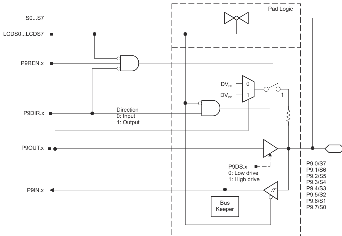
9-13. Port P9 (P9.0 to P9.7) Diagram
