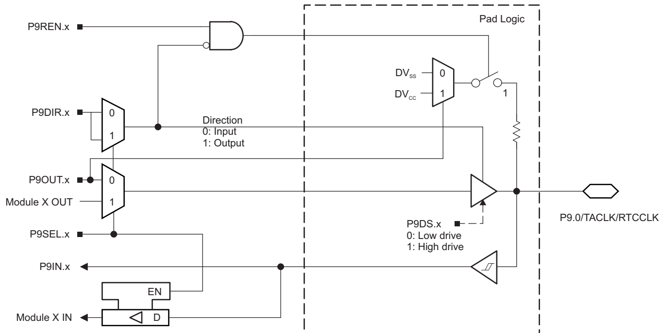
6-11. Port P9 (P9.0) Diagram (MSP430F67xxIPZ Only)
