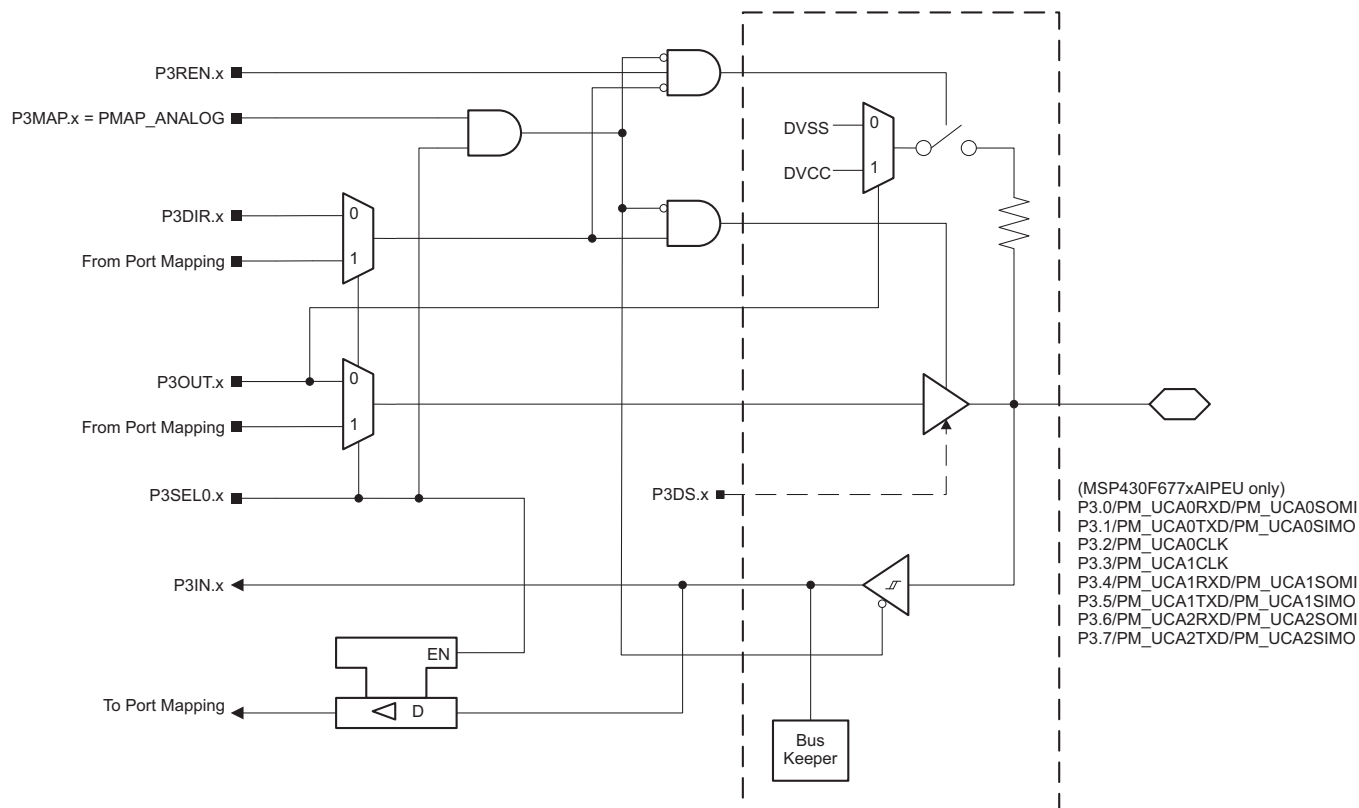
Figure 6-14. Ports P3 (P3.0 to P3.7) Diagram (PEU Package Only)
