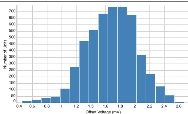
8-25. OA Offset Voltage Sample Production Distribution
