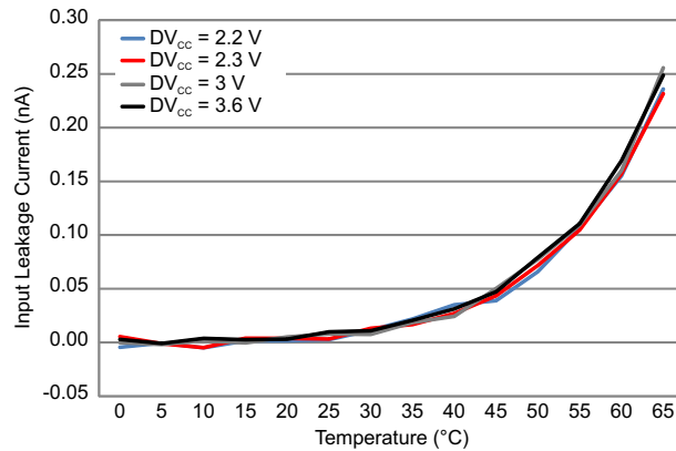
8-28. OA Switch Input Leakage Current vs Temperature
