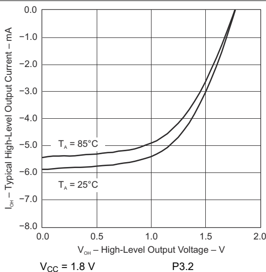
8-6. Typical High-Level Output Current Vs High-Level Output Voltage
