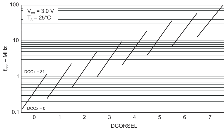
図 8-2. Typical DCO Frequency
