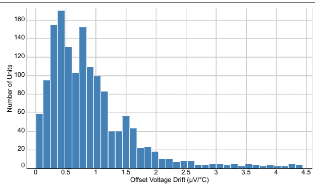
8-26. OA Offset Voltage Drift Sample Production Distribution
