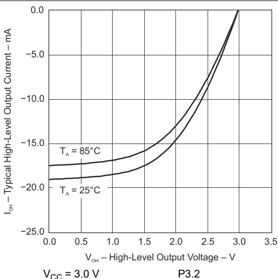
8-5. Typical High-Level Output Current Vs High-Level Output Voltage
