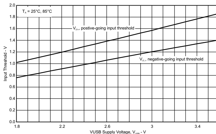
FIG 8-32. Ports PU.0, PU.1 Typical Input Threshold Characteristics
