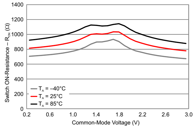
8-29. OA Switch R ON vs Common-Mode Voltage
