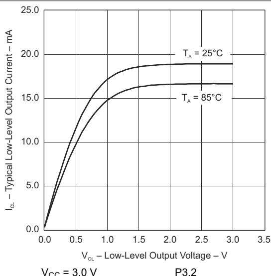
8-3. Typical Low-Level Output Current vs Low-Level Output Voltage
