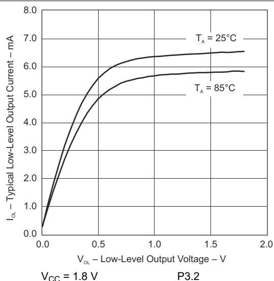
8-4. Typical Low-Level Output Current vs Low-Level Output Voltage
