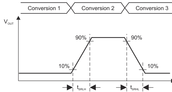
8-22. Slew Rate Testing
