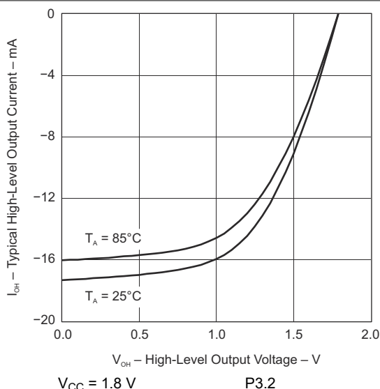
8-10. Typical High-Level Output Current vs High-level Output Voltage
