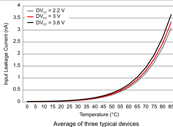
8-27. Ground Switch Input Leakage Current vs Temperature
