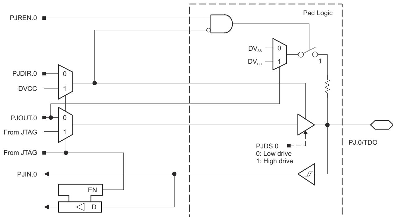
9-25. Port PJ (PJ.0) Diagram
