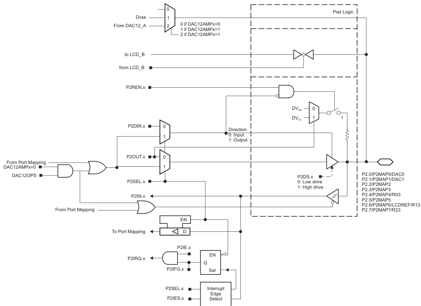
9-4. Port P2 (P2.0 to P2.7) Diagram
