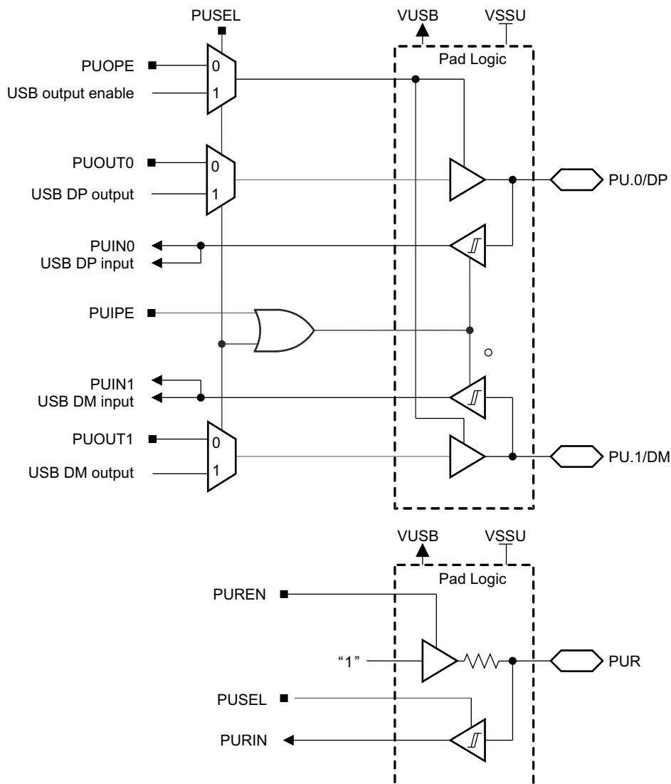
9-24. Port U (PU.0 and PU.1) Diagram
