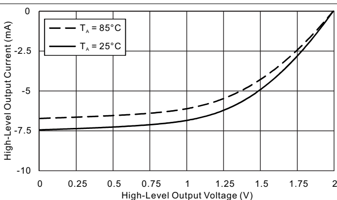
Figure 5-8. Typical High-Level Output Current vs High-Level Output Voltage (DVCC = 2 V)
