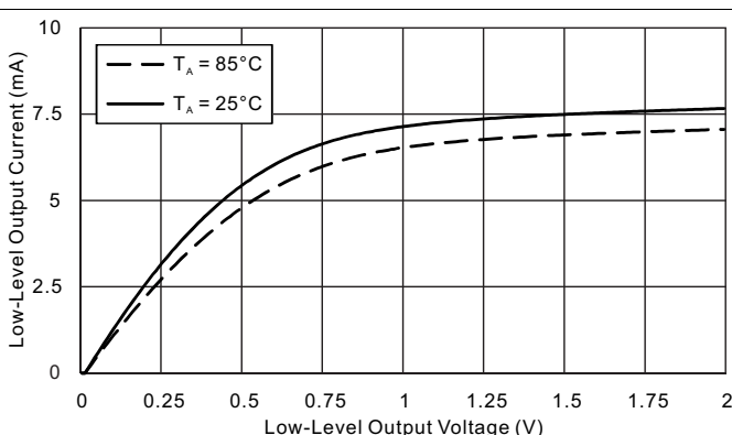
Figure 5-6. Typical Low-Level Output Current vs Low-Level Output Voltage (DVCC = 2 V)
