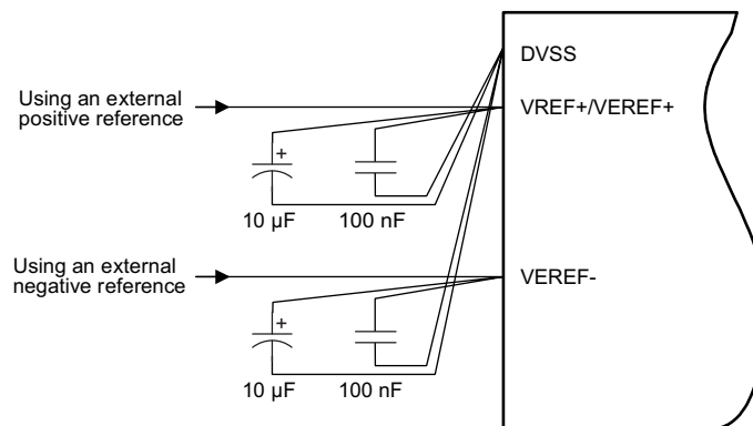
✎ 7-5. ADC Grounding and Noise Considerations
