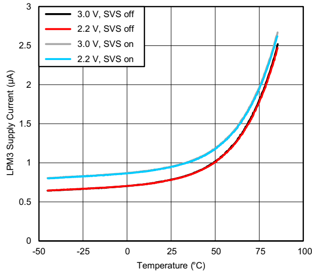
Figure 8-2. LPM3 Supply Current vs Temperature (LPM3,XT3.7)
