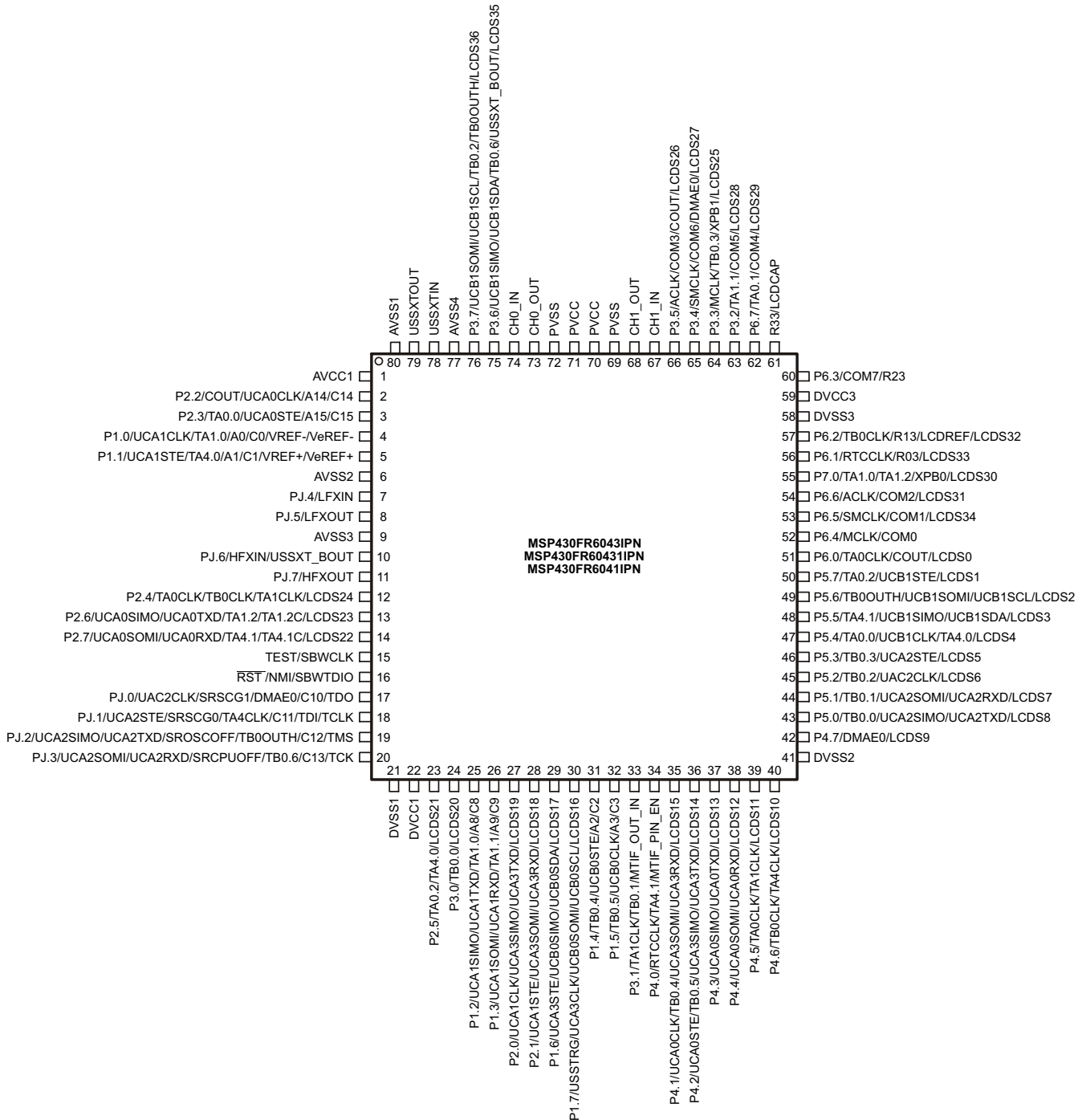
7-1. 80-Pin PN Package (Top View)
