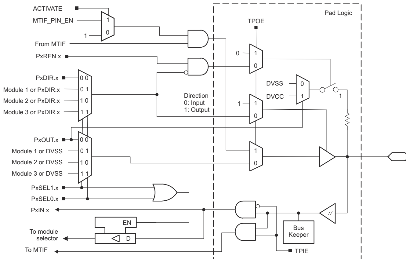
Figure 9-11. Port P3 (P3.1) Diagram
