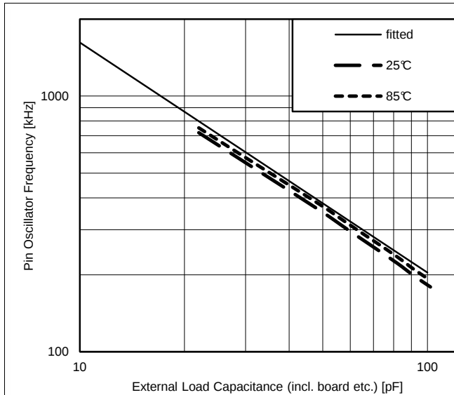
Figure 5-12. Typical Oscillation Frequency vs Load Capacitance
