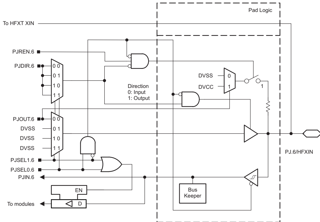
☒ 6-11. Port PJ (PJ.6) Diagram
