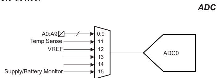
図 8-1. Analog Connections
