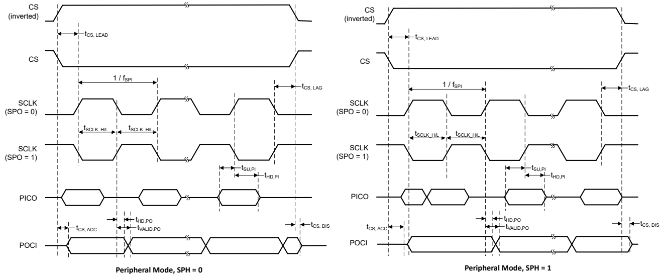
図 7-5. SPI Timing Diagram - Peripheral Mode
