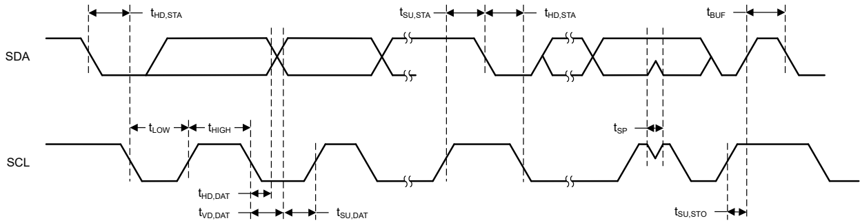
図 7-3. I2C Timing Diagram
