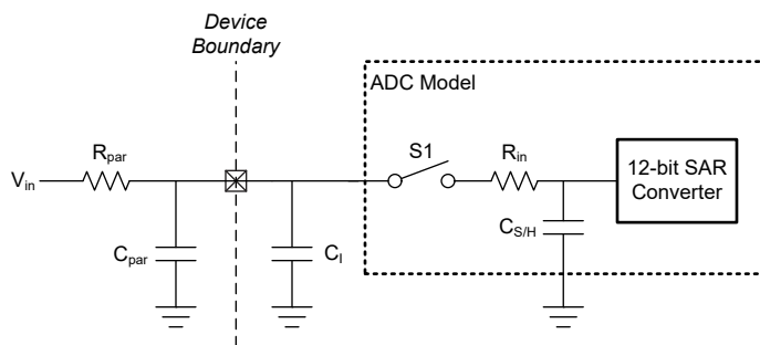
FIG 7-2. ADC Input Network
