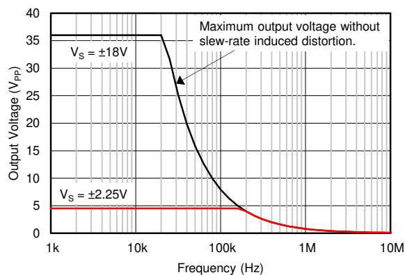
FIG 6-37. Maximum Output Voltage Amplitude vs Frequency
