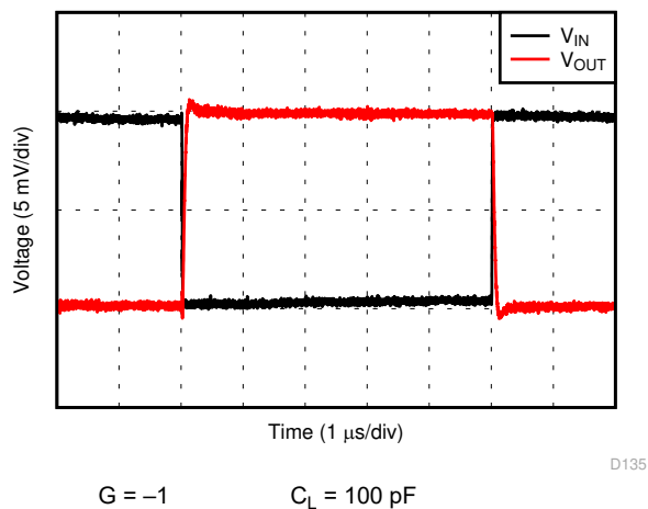
6-24. Small-Signal Step Response (100 mV)
