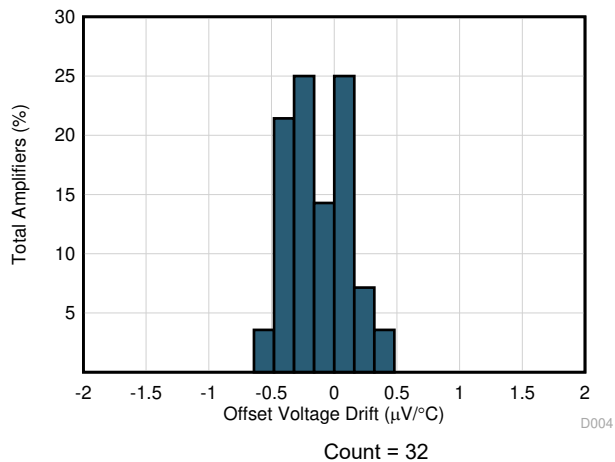
6-20. Input Offset Voltage Drift Distribution
