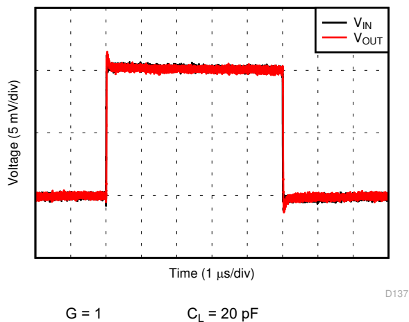
6-23. Small-Signal Step Response (100 mV)
