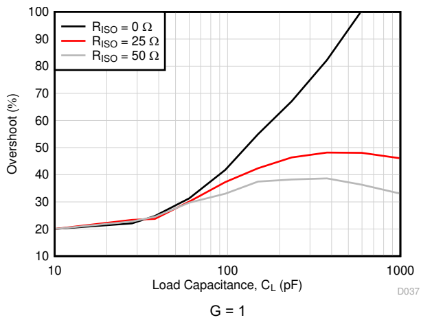
FIG 6-36. Percent Overshoot vs Capacitive Load
