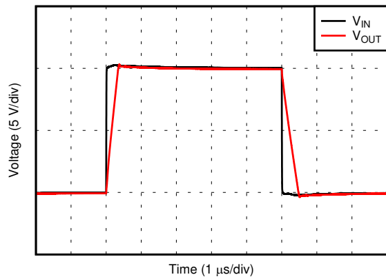
FIG 6-25. Large-Signal Step Response
