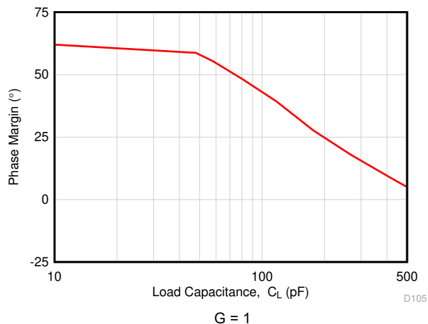
FIG 6-35. Phase Margin vs Capacitive Load
