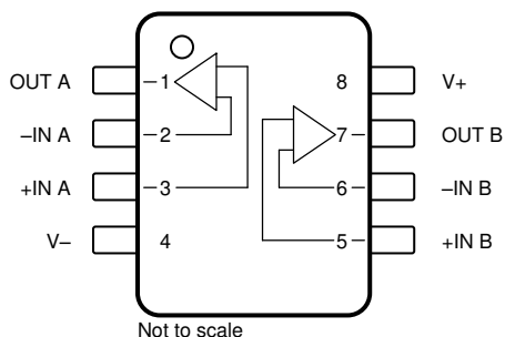
FIG 5-3. OPA1656 D (8-Pin SOIC) Package, Top View
