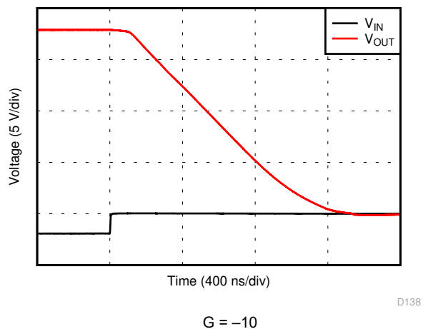
FIG 6-39. Positive Overload Recovery
