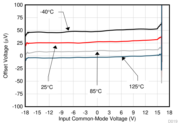
6-22. Input Offset vs Common Mode Voltage
