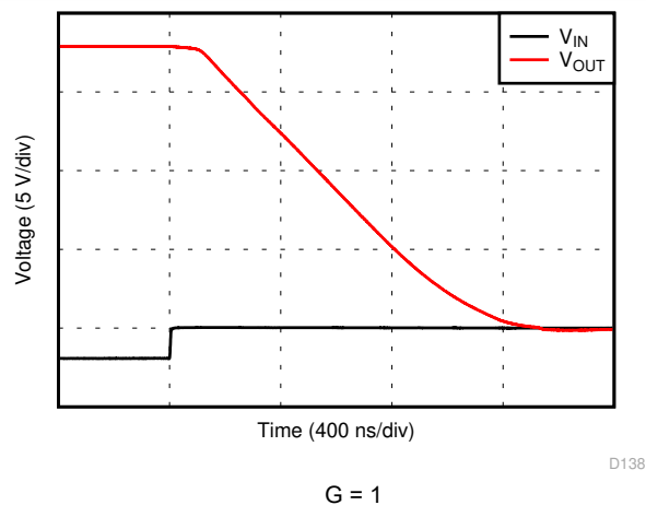
FIG 6-41. No Phase Reversal
