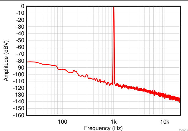
Figure 8-5. Output Spectrum for a 10-mV RMS , 1-kHz Input Signal
