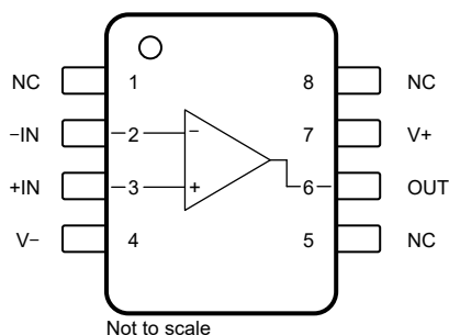
FIG 5-1. OPA1655 D (8-Pin SOIC) Package, Top View
