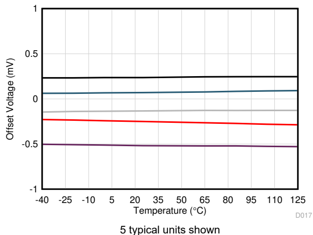
6-21. Input Offset vs Temperature
