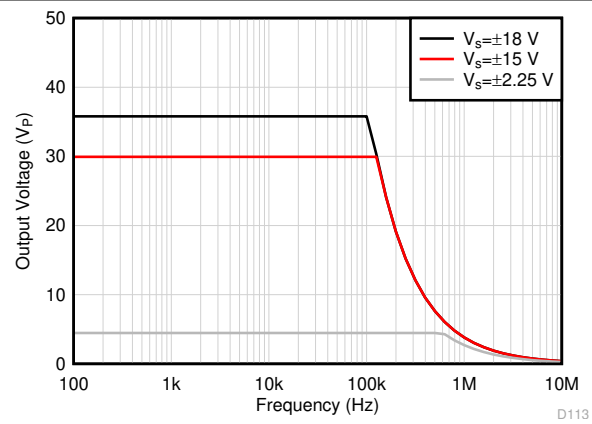
图 6-4. Maximum Output Voltage vs Frequency
