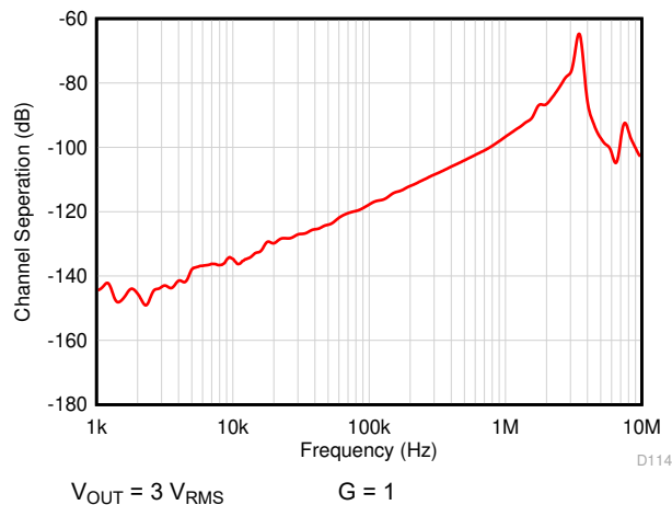
FIG 6-15. Channel Separation vs Frequency
