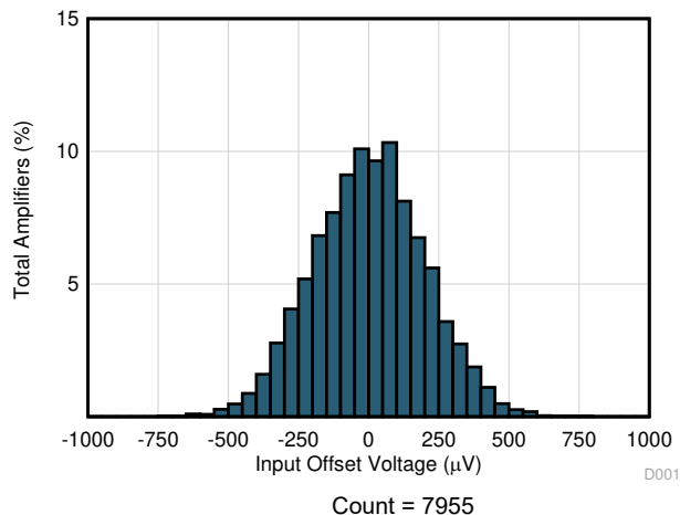
6-19. Input Offset Voltage Distribution
