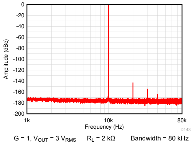
FIG 6-13. FFT, 10-kHz Sine Wave
