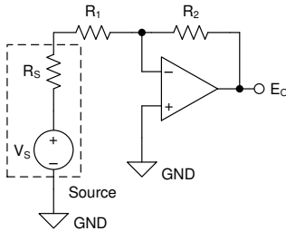
(B) Noise in Inverting Gain Configuration
