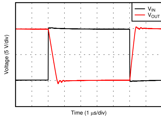
FIG 6-26. Large-Signal Step Response
