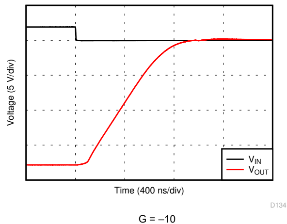
FIG 6-38. Negative Overload Recovery
