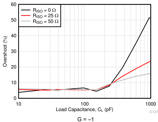
FIG 6-37. Percent Overshoot vs Capacitive Load
