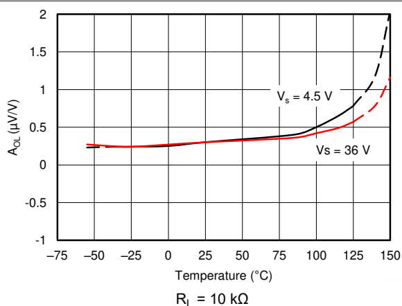
7-23. Open-Loop Gain vs Temperature
