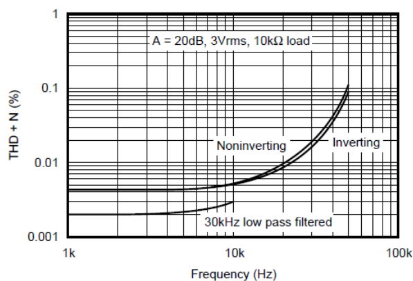
図 6-1. Total Harmonic Distortion and Noise vs Frequency
