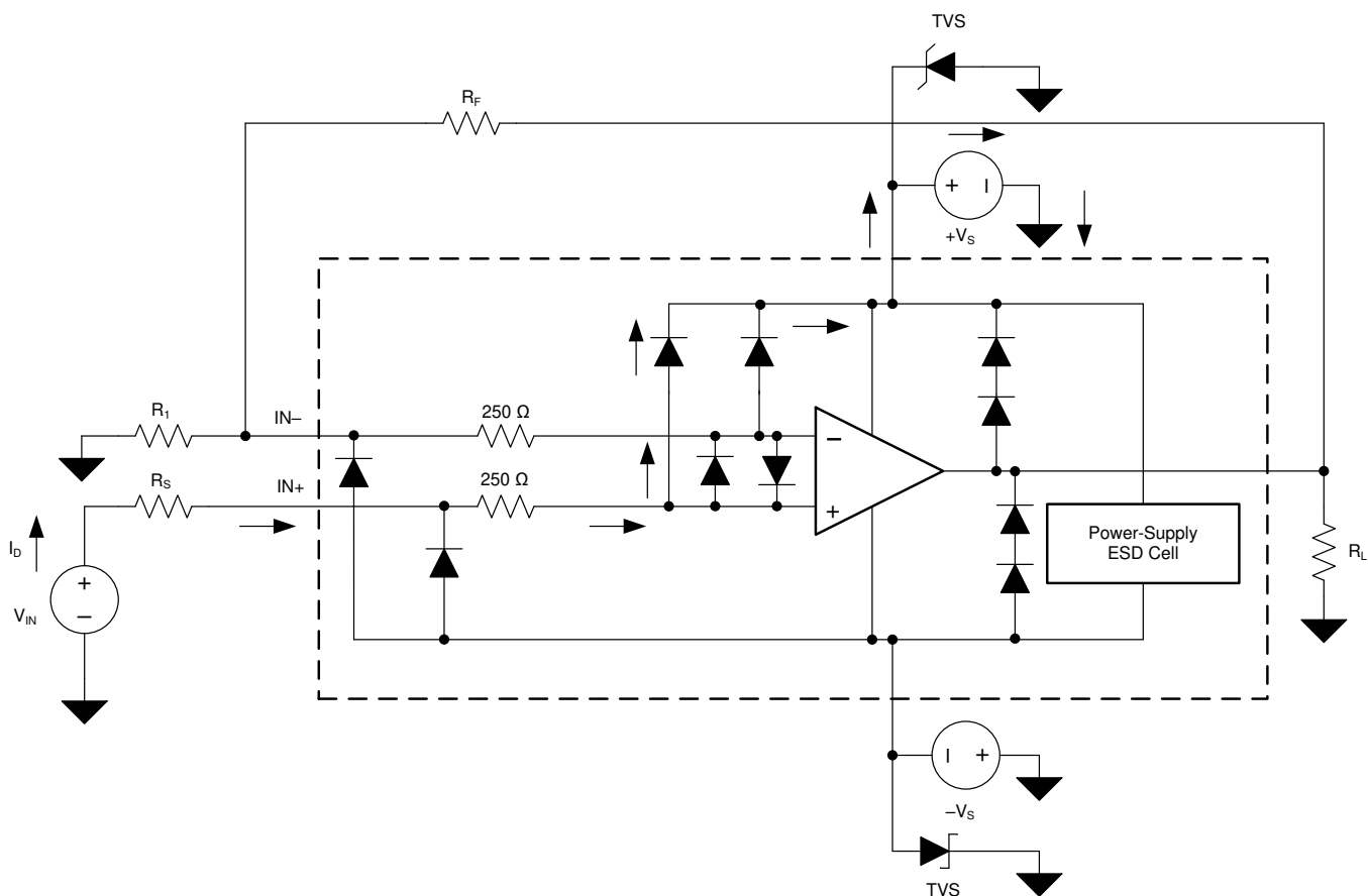
FIG 43. Equivalent Internal ESD Circuitry Relative to a Typical Circuit Application
