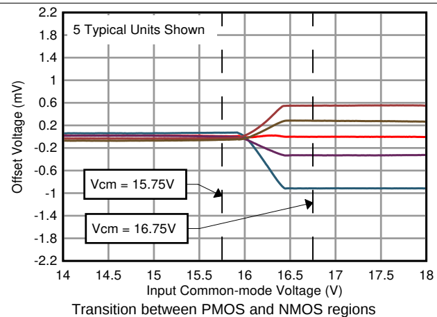
Figure 6. Offset Voltage vs Common-Mode Voltage in Transition Region
