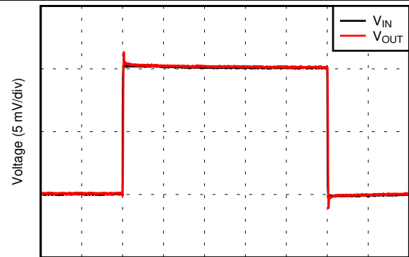
FIG 32. Negative Overload Recovery
