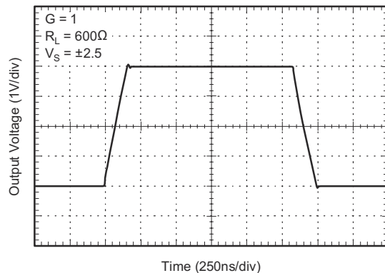
7-19. Large-Signal Step Response
