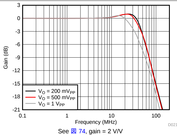
Figure 21. Noninverting Large-Signal Bandwidth vs V_{OPP}
