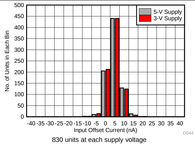
FIG 44. Input Offset Current Distribution
