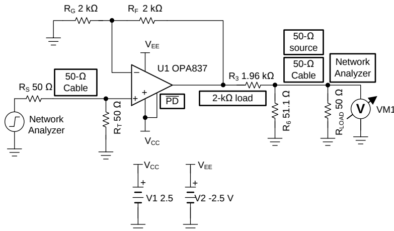
図 74. Characterization Test Circuit for Network, Spectrum Analyzer
