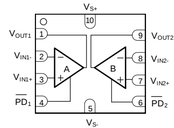
OPA2837 RUN Package 10-Pin WQFN Top View
