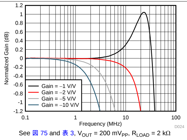
Figure 24. Inverting Response Flatness vs Gain
