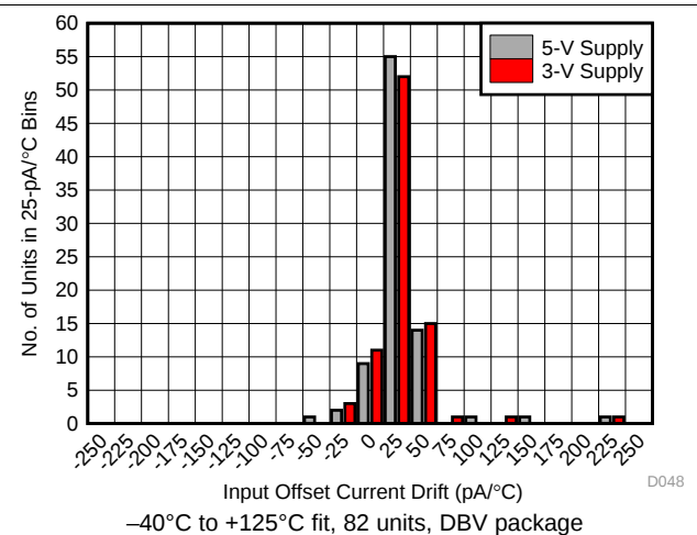
FIG 48. Input Offset Current Drift Distribution
