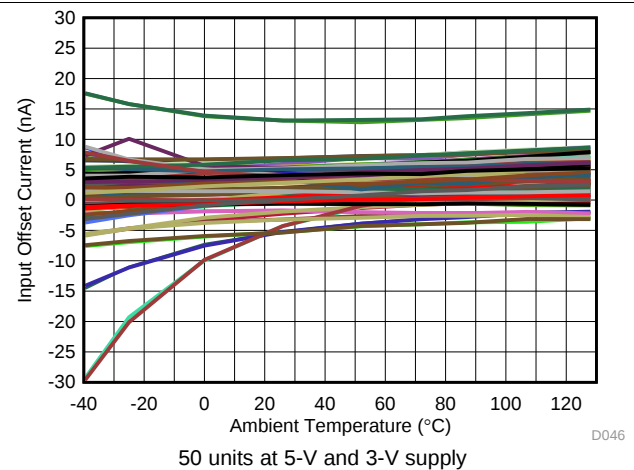
FIG 46. Input Offset Current vs Ambient Temperature
