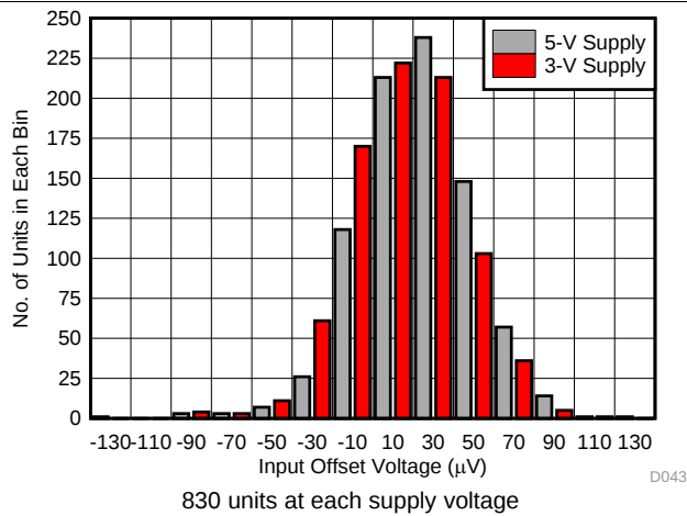
FIG 43. Input Offset Voltage Distribution
