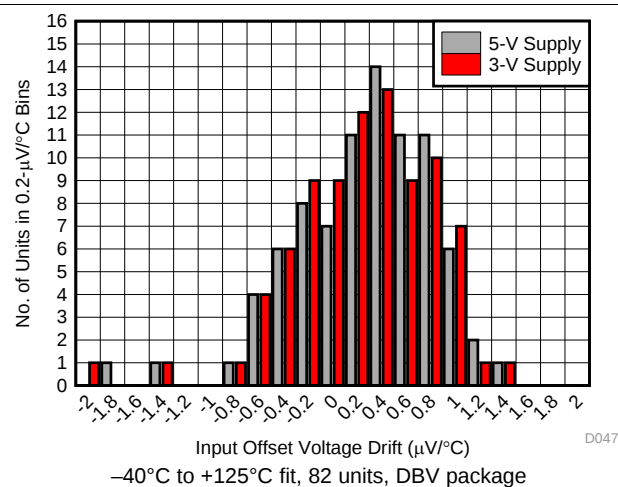
FIG 47. Input Offset Voltage Drift Distribution
