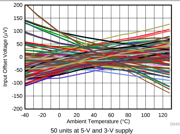
FIG 45. Input Offset Voltage vs Ambient Temperature
