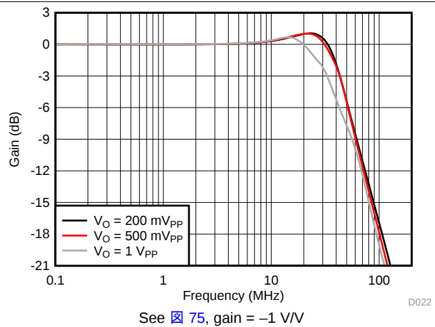
Figure 22. Inverting Large-Signal Bandwidth vs V_{OPP}
