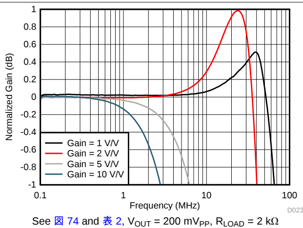
Figure 23. Noninverting Response Flatness vs Gain
