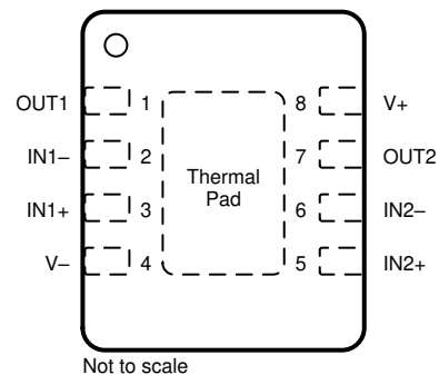
図 5-5. OPA2991 DSG Package (A) 8-Pin WSON With Exposed Thermal Pad (Top View)
