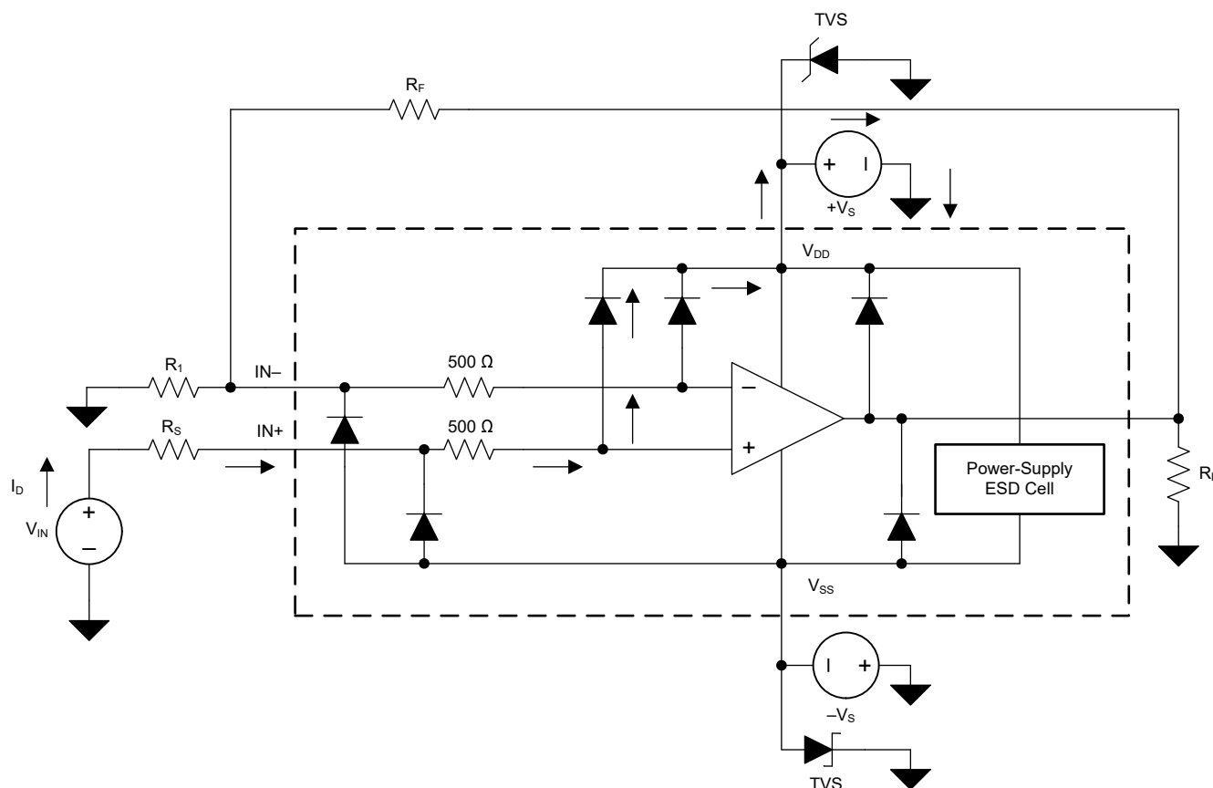
FIG 7-10. Equivalent Internal ESD Circuitry Relative to a Typical Circuit Application
