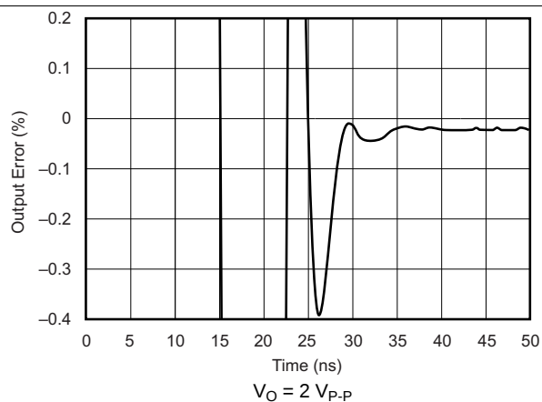
Figure 27. Output Settling Time to 0.1%
