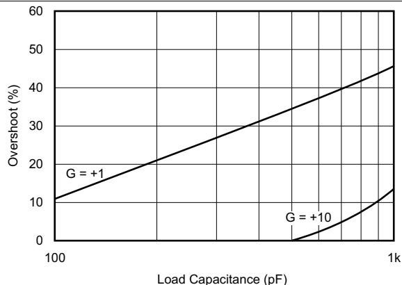
Figure 13. Small-Signal Overshoot vs Load Capacitance
